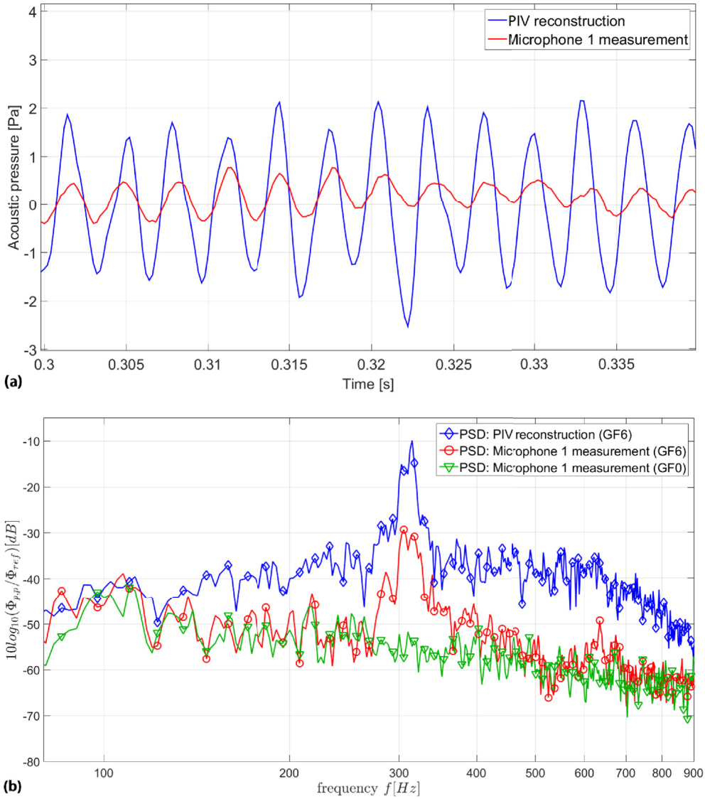
Fig. 9. Time series (a) and power spectra with \Delta f = 2.4\text{ Hz} (b) of far-field acoustic pressure evaluated by compact formulation of Curle's analogy based on full span coherence assumption from PIV measurements in comparison with the simultaneous microphone measurement at the location of Microphone 1. The reference value \Phi_{ref} = 1 \text{ Pa}^2 \cdot \text{s} . GF6: 6% c Gurney flap mounted on the trailing edge. GF0: clean NACA 0015 configuration (no Gurney flap).
