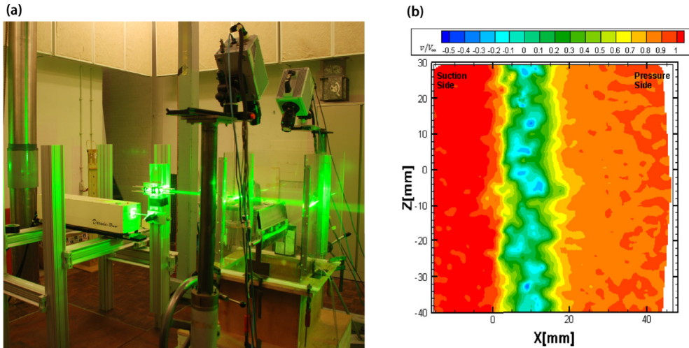
Fig. 11. Experimental setup for spanwise coherence length measurements (a) and a snapshot of instantaneous streamwise velocity component in the streamwise-spanwise plane ( x - z ) 5 mm downstream of the airfoil trailing edge (b).
