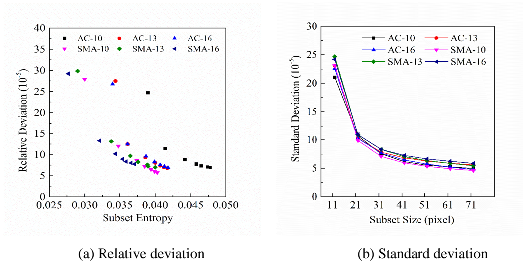
Fig.6 Relation between relative deviation, standard deviation and subset size
