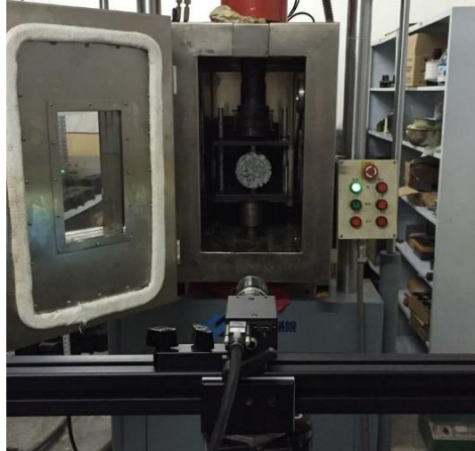
Fig.1 Test equipment in this research
