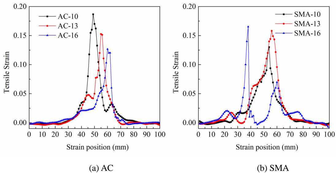
Fig.8 Horizontal tensile strain distribution of different mixtures
