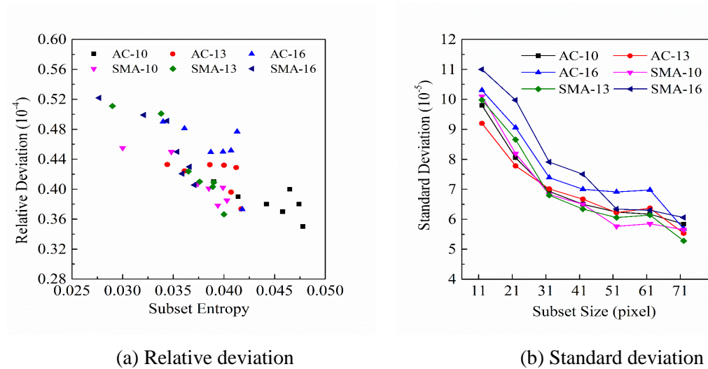
Fig.4 Relation between relative deviation, standard deviation and subset size
