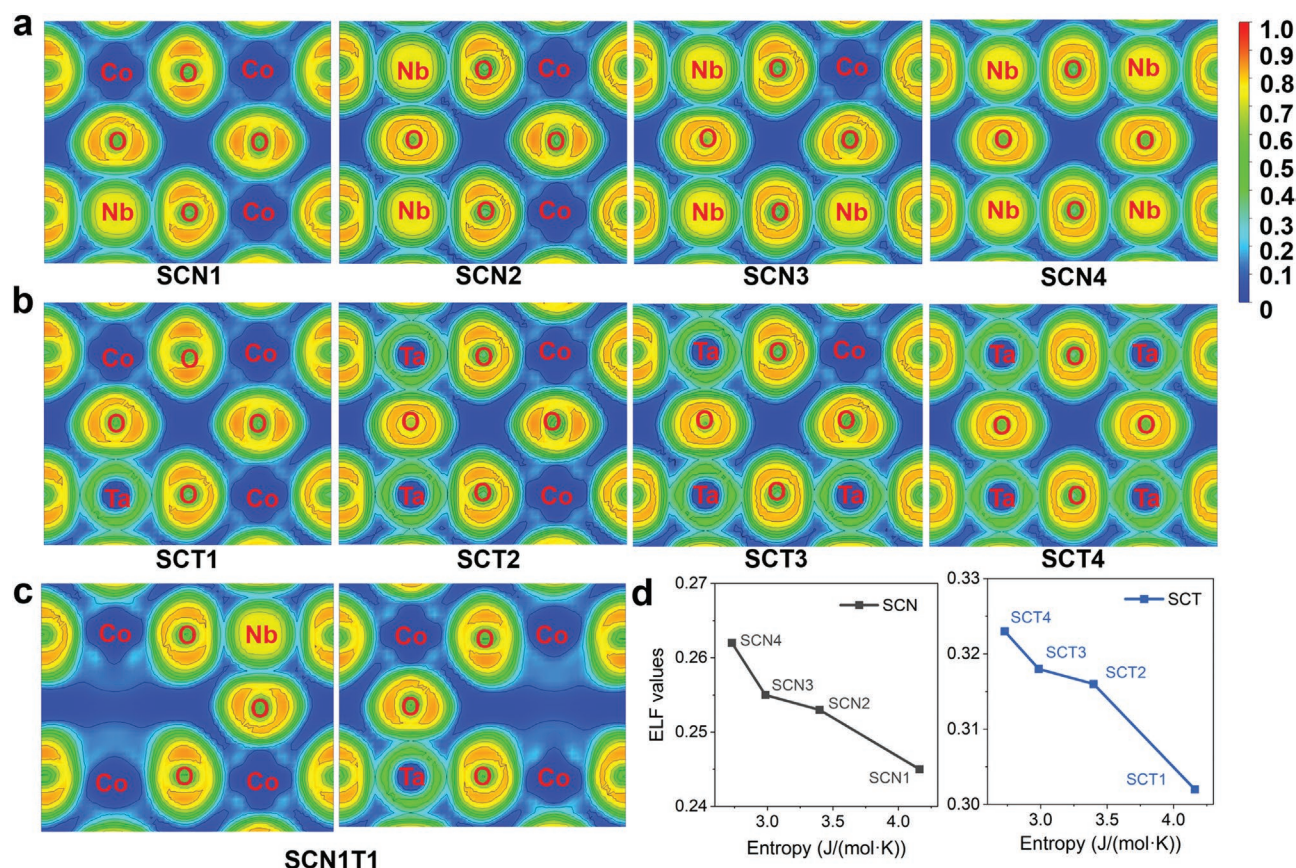
Figure 5. ELF maps for model (001) planes of a) SCN, b) SCT, and c) SCNT. The \text{BO}_6 octahedron contains six B-O bonds, the ELF values for which are obtained by combining the ELF values for the (100) and (001) planes. d) Variation of ELF values along dopant-oxygen bonds shown for various SCN and SCT models with differing configuration entropy. Models are shown in Figures S7–S9 (Supporting Information). Lines through the points are guides to the eye.
