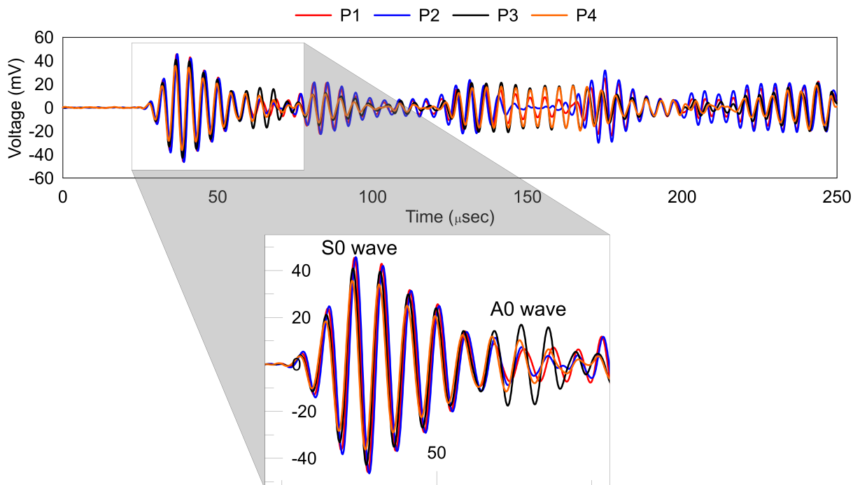
Figure 5: GW measurements at 4 wavelengths with single excitation at 250 kHz
