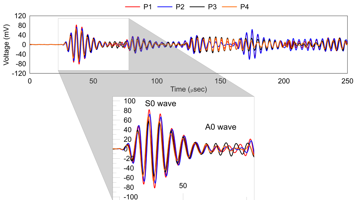
Figure 6: GW measurements at 4 wavelengths with inphase excitation at 250 kHz
