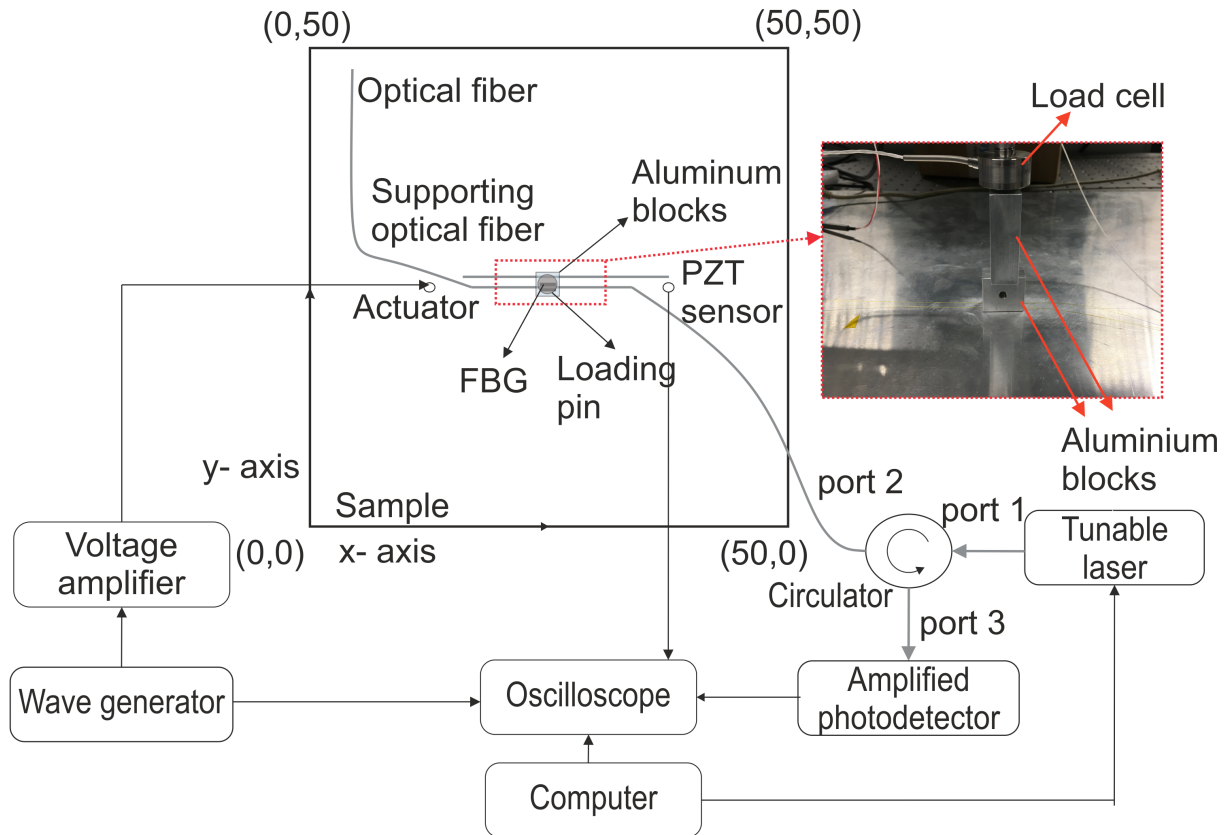
Figure 2: Schematic for the experimental setup
