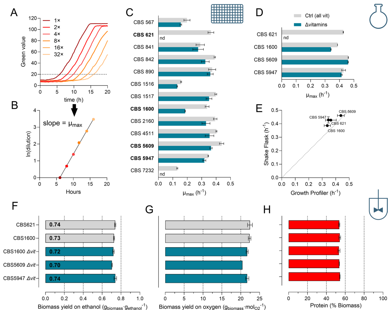
Fig. 4 Characterization of C. jadinii strains in microtiter plates, shake flasks and bioreactors concerning vitamin dependency. A Representative growth curves of serially diluted CBS 621 in microtiter plates, ranging from 1 to 32× dilution, initial OD 660 0.2 to 0.00625, respectively. B Calculation of specific growth rates via serial dilution method. The time (h) required for a specific dilution to reach a green value of 20 was plotted against the natural logarithm of the respective dilution (1–32). C Specific growth rates for 13 C. jadinii strains grown on ethanol in the presence or absence of vitamins, calculated with the serial dilution method, nd non-detectable. D Specific growth rates of 4 C. jadinii strains grown on ethanol in shake flasks in the presence or absence of vitamins. E Correlation of specific growth rates obtained in microtiter plates (x-axis) with those measured in shake flasks (y-axis) for strains grown in the presence of vitamins. F–H Biomass yields on ethanol, oxygen and protein content for selected strains grown in ethanol-limited chemostats (dilution rate 0.10 h -1 ). Where indicated by Δvit, no vitamins were added to the cultivation, n = 2–3
