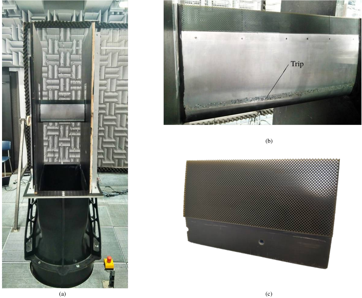
Fig. 2 (a) Overall view of the contraction with the airfoil and the side plates, and the microphone array on the back. (b) Detail view of the airfoil with a 3D-printed insert. (c) Detail of 3D-printed insert with l_h = 1.5 mm. Total length is 6 cm. Only the last 4 cm of insert are exposed to the flow.
