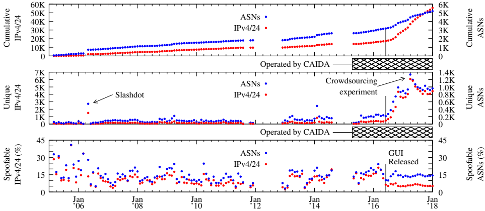
Figure 2.1: Overview of Spoofer project data collection over time, aggregated per month. The gaps are due to hardware failures. Between November 2016 and December 2017, the range of spoofable IPv4 prefixes is 4.9% – 6.8%, and the range of spoofable ASNs is 13.1% – 14.5%. The two data collection peaks in April and May 2017 are due to the crowdsourcing experiments in this study, and those results are qualitatively similar to those collected between November 2016 and December 2017.
