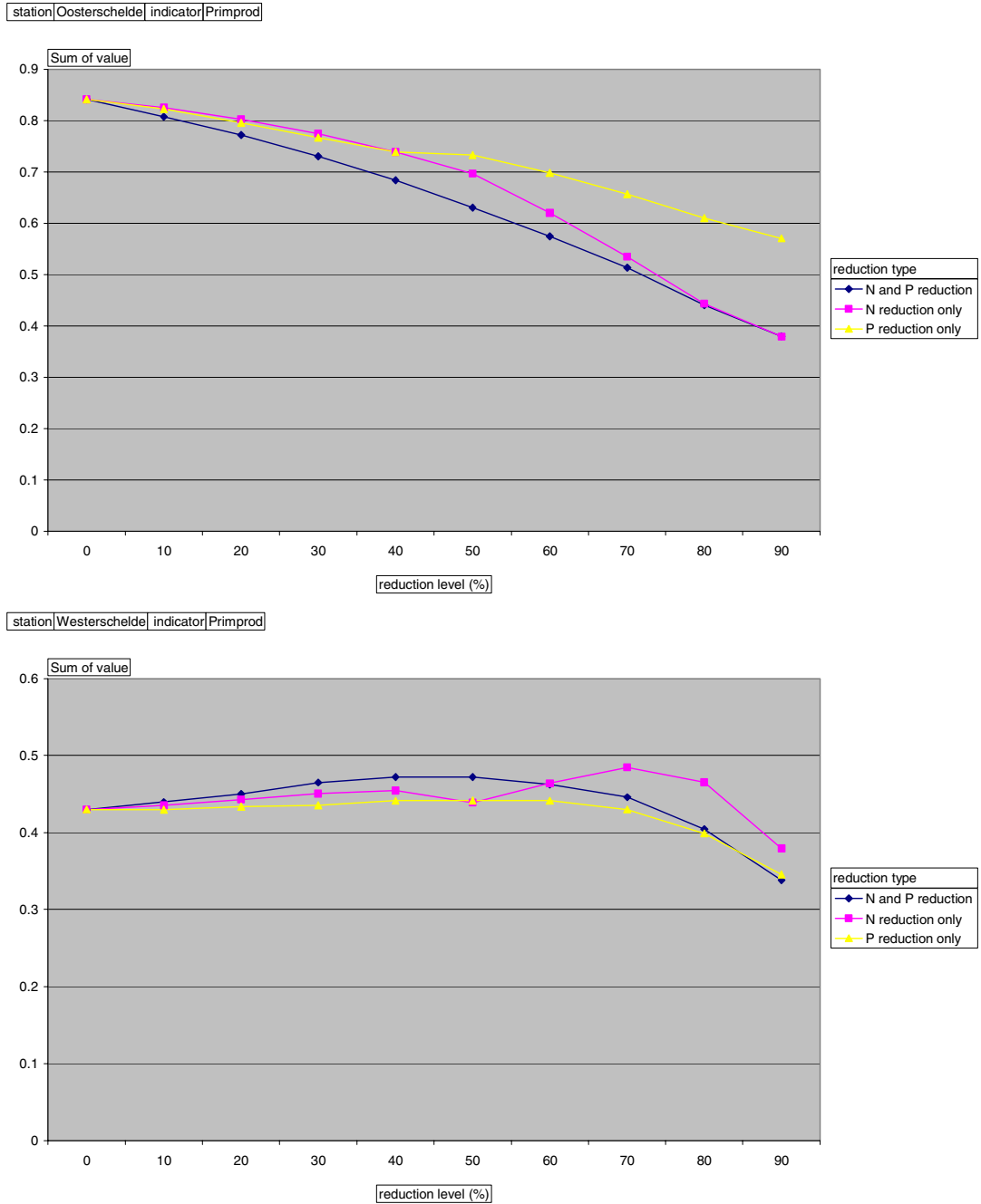
Figure C.3b: Response curves for yearly averaged primary production ( gC/m^3.d ) concentrations in the areas Oosterschelde and Westerschelde
