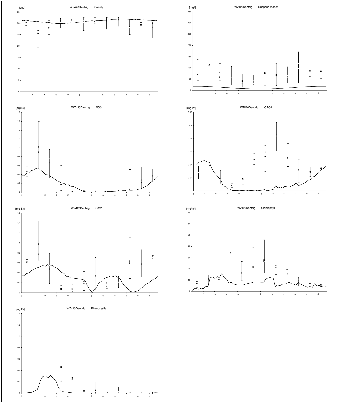
Figure A.13: Model results for the average year and average (square), median (circle) and 90 percentile of field observations of 1995 – 1998 at station Dantziggat.
