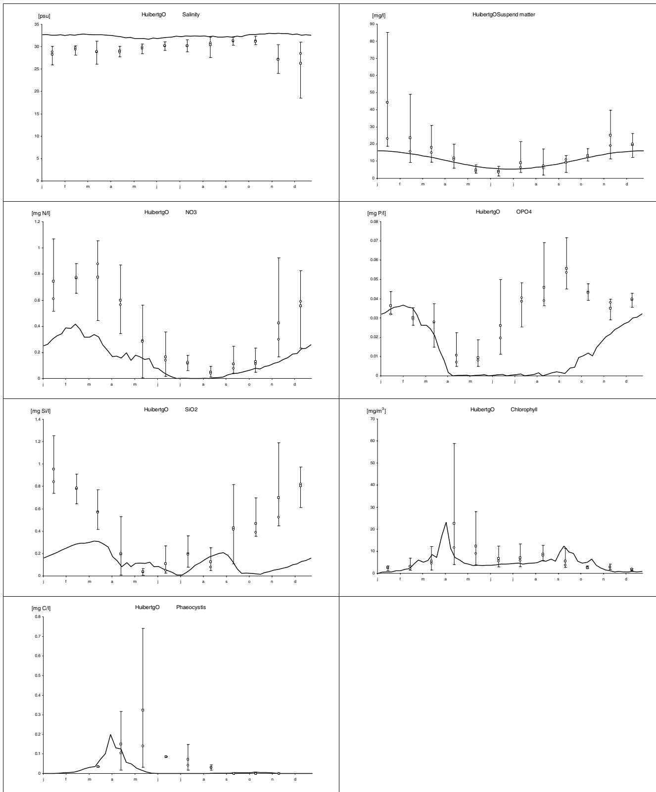
Figure A.9: Model results for the average year and average (square), median (circle) and 90 percentile of field observations of 1995 – 1998 at station Huibertgat Oost.
