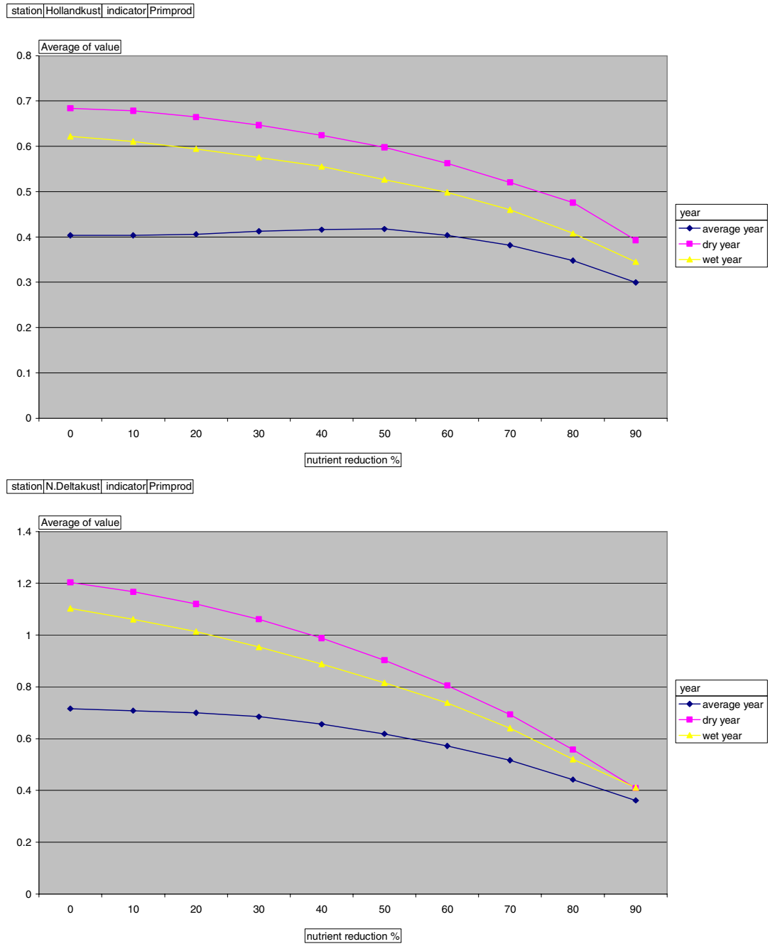
Figure B.6a: Response curves for yearly averaged primary production (gC/m 3 .d) concentrations in the areas Delta coast and Holland coast
