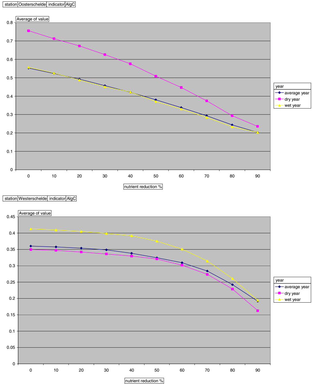
Figure B.5b: Response curves for summer averaged algal biomass ( gC/m^3 ) concentrations in the areas Oosterschelde and Westerschelde
