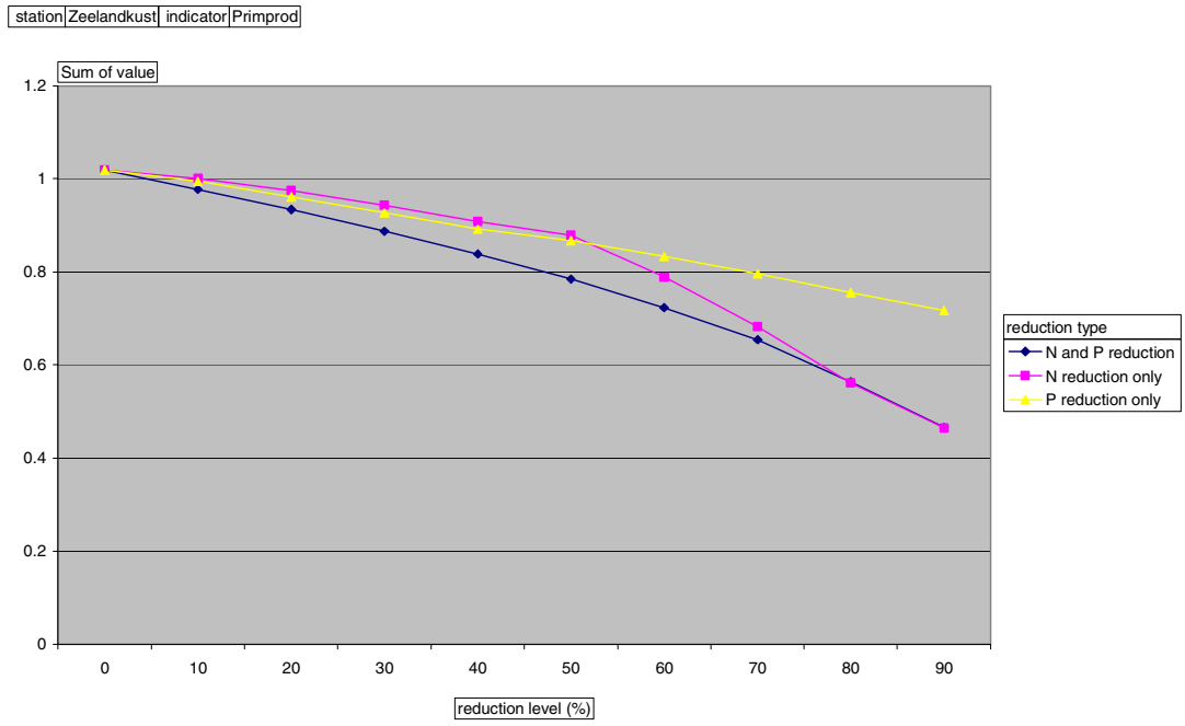
Figure C.3d: Response curves for yearly averaged primary production ( \text{gC}/\text{m}^3 \cdot \text{d} ) concentrations in the Zeeland coast area.
