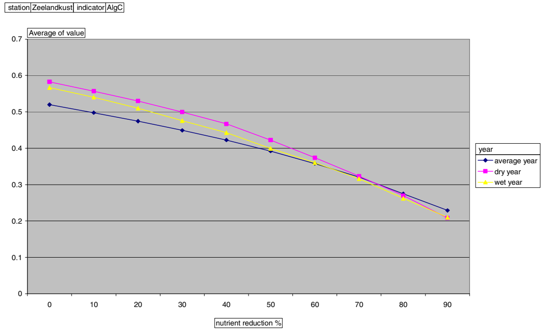
Figure B.5d: Response curves for summer averaged algal biomass ( \text{gC}/\text{m}^3 ) concentrations in the Zeeland coast area.
