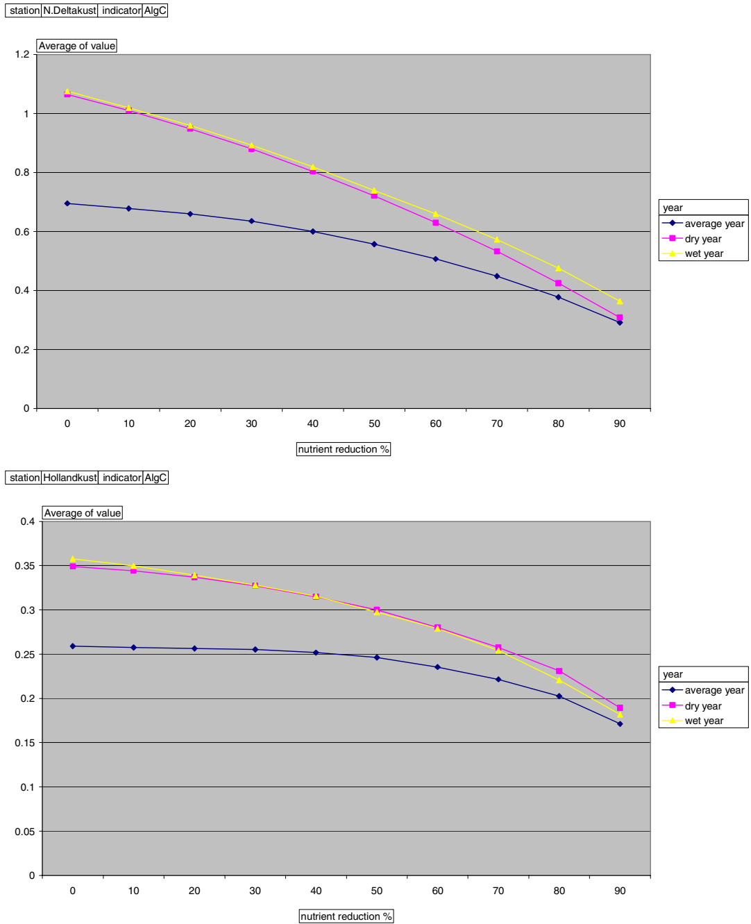
Figure B.5a: Response curves for summer averaged algal biomass ( gC/m^3 ) concentrations in the areas Delta coast and Holland coast
