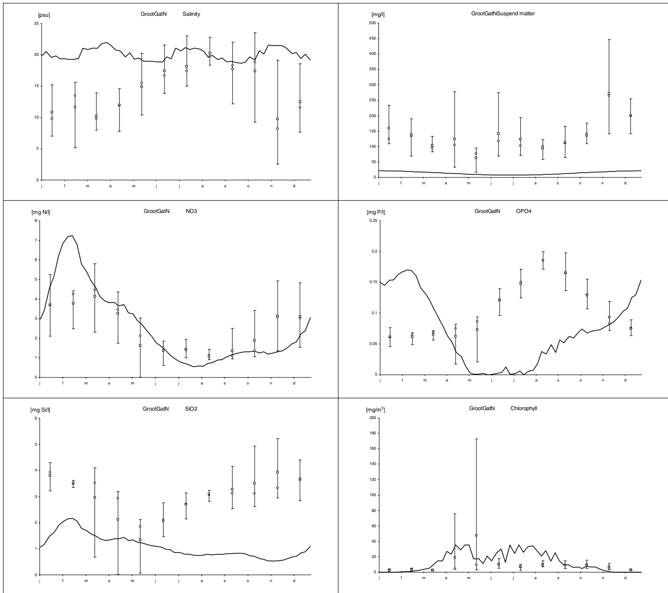
Figure A.14: Model results for the average year and average (square), median (circle) and 90 percentile of field observations of 1995 – 1998 at station Groot Gat Noord.
