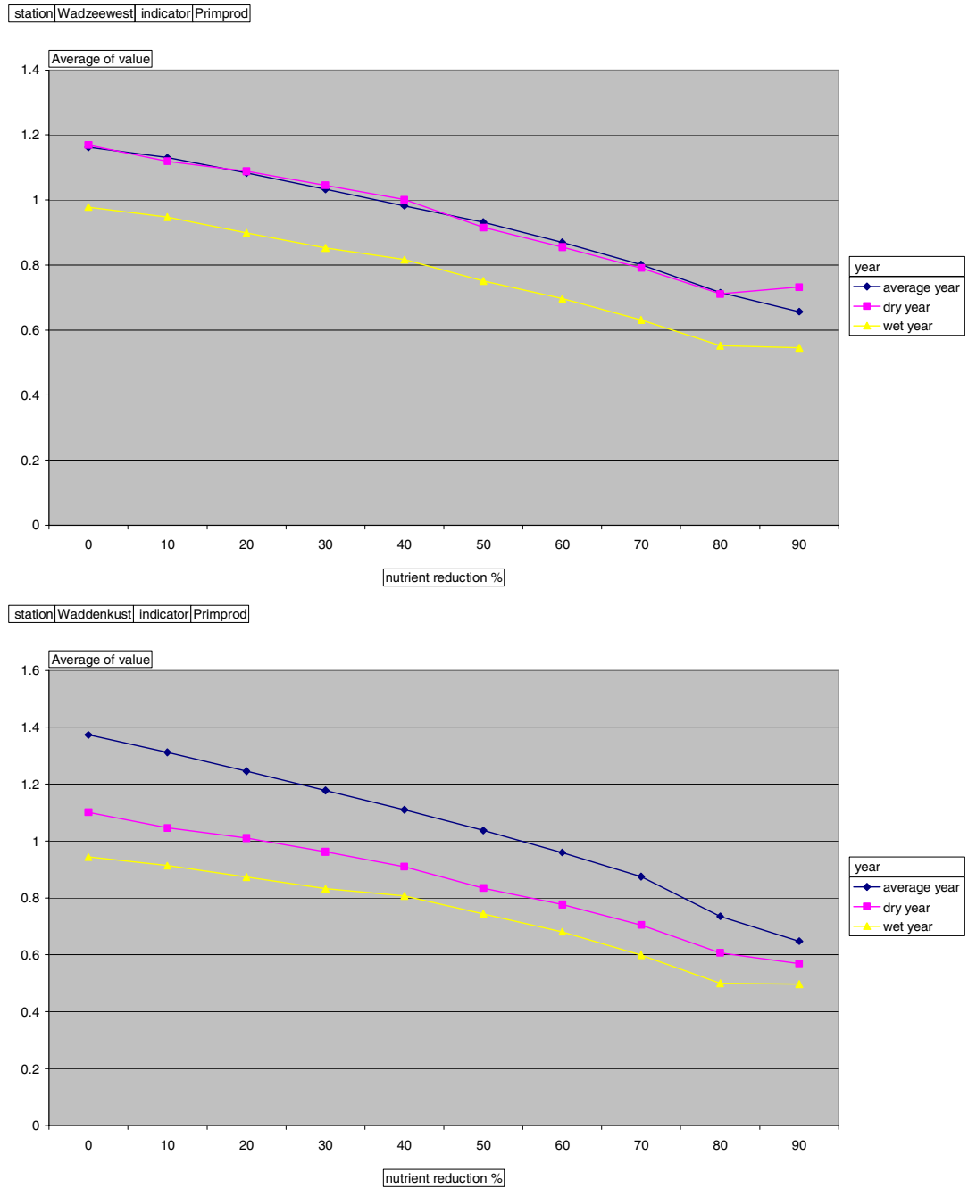
Figure B.6c: Response curves for yearly averaged primary production ( \text{gC}/\text{m}^3 \cdot \text{d} ) concentrations in the areas western Wadden Sea and Wadden coast.
