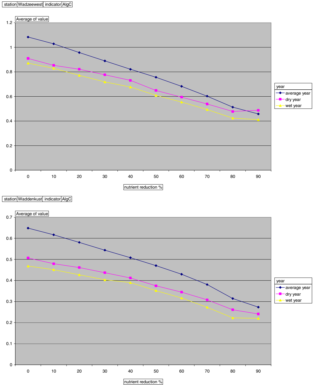
Figure B.5c: Response curves for summer averaged algal biomass (gC/m 3 ) concentrations in the areas western Wadden Sea and Wadden coast.
