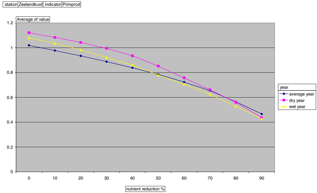
Figure B.6d: Response curves for yearly averaged primary production ( \text{gC}/\text{m}^3 \cdot \text{d} ) concentrations in the Zeeland coast area.
