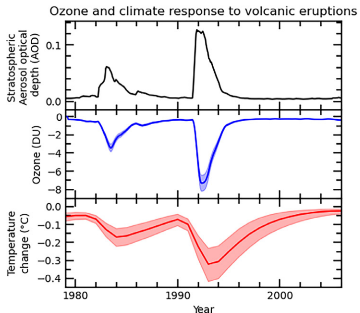
FIG. 10. Time series of SAOD, the anomaly in TCO ( \Delta O_3 ) between 60°S and 60°N, and the anomaly in GMST ( \Delta T ) following the volcanic eruptions of El Chichón and Mount Pinatubo in 1982 and 1991, respectively. The monthly SAOD time series is based on integration of extinction coefficients from the GloSSAC v2 database (Thomason et al. 2018; Kovilakam et al. 2023). The \Delta O_3 time series is the computed impact of SAOD on \Delta O_3 found for a multiple linear regression of monthly TCO averaged over 60°S–60°N vs the following terms: equivalent effective stratospheric chlorine for 3-yr-old air, total solar irradiance, SAOD, the QBO in the zonal-mean wind in the tropical lower stratosphere, and El Niño–Southern Oscillation, as in Fig. 3-1 of Chipperfield et al. (2007). The \Delta O_3 time series is smoothed with a 6-month running mean; the shaded region defines the 2\sigma uncertainty based on a conditional regression. The time series of \Delta T and the 2\sigma uncertainties represented by the shaded region are obtained from the model output used to construct Fig. 7.8 of the IPCC Sixth Assessment Report (IPCC 2021).
