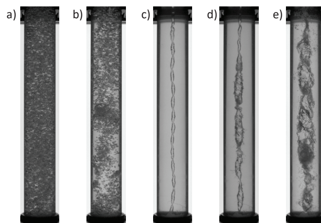
Figure 2: Gas-liquid swirl flow patterns. a) weak swirling bubbly, b) swirling bubbly with bubble agglomeration, c) stable column, d) pulsating column and e) unstable column.
