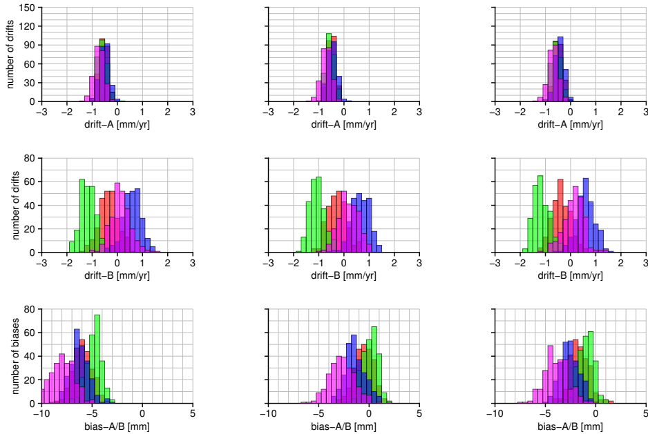
Figure 5.9: Histograms of the TOPEX A&B drifts and intramission bias for the four averaging methods based on model 3 without cal-1 applied to TOPEX-A&B. On the left, at the middle and on the right the histograms for the bm4, CSR and CLS SSB corrections. In red, green, blue and purple the methods m1, m2, m3 and m4, respectively.
