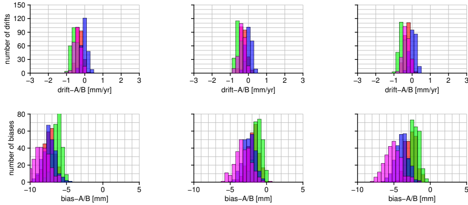
Figure 5.8: Histograms of the TOPEX A/B drift and intramission bias for the four averaging methods based on model 2 without cal-1 applied to TOPEX-A&B. On the left, at the middle and on the right the histograms for the bm4, CSR and CLS SSB corrections. In red, green, blue and purple the methods m1, m2, m3 and m4, respectively.
