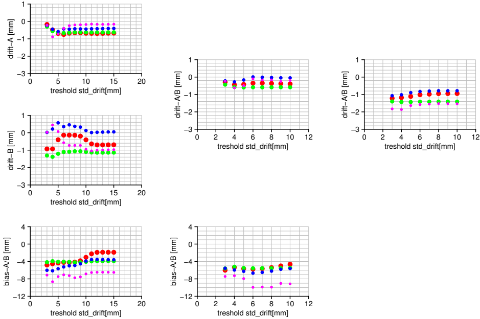
Figure 5.11: Sensitivity of the four averaging methods m1 (red), m2 (green), m3 (blue) and m4 (pink) to the threshold for the trend uncertainties. On the left separate drifts are estimated for TOPEX-A&B and an intramission bias (model 3), in the center one drift for TOPEX is estimated and an intramission bias (model 2) and on the right only one drift is estimated (model 1).
