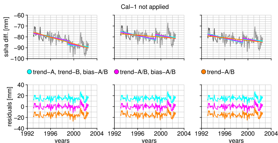
Figure 5.3: Top: time series of sea surface height differences (TOPEX-ERS1&2) for the bm4 (left), CSR (middle) and the CLS (right) SSB models for which Cal-1 is removed, together with three models fitted to the data. Bottom: residuals after subtracting the models.
