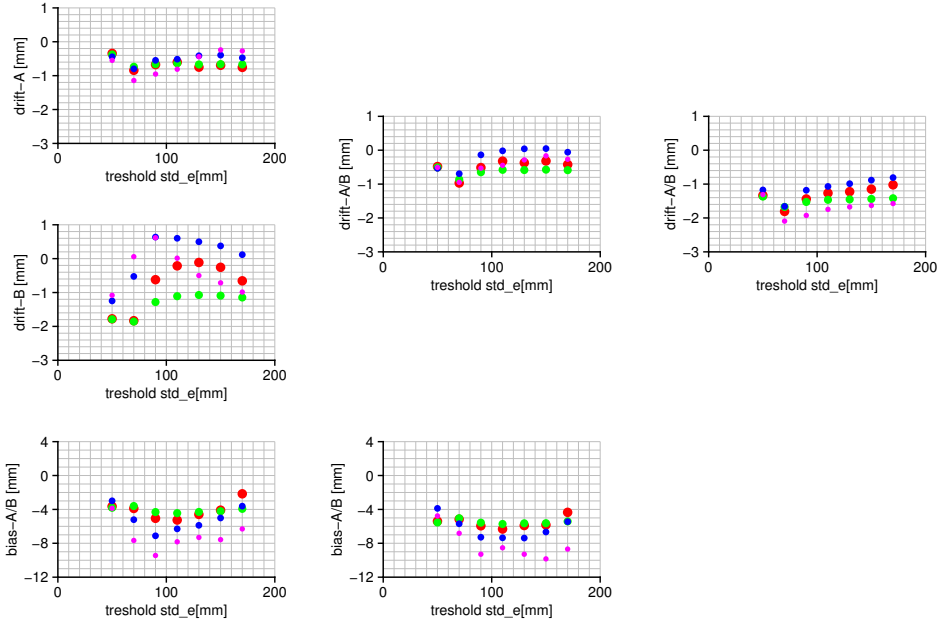
Figure 5.10: Sensitivity of the four averaging methods m1 (red), m2 (green), m3 (blue) and m4 (pink) to the threshold for the standard deviation of the residuals. On the left separate drifts are estimated for TOPEX-A&B and an intramission bias (model 3), in the center one drift for TOPEX is estimated and an intramission bias (model 2) and on the right only one drift is estimated (model 1).
