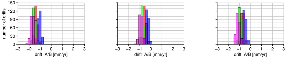
Figure 5.7: Histograms of the TOPEX A/B drift for the four averaging methods based on model 1 without cal-1 applied to TOPEX-A&B. On the left, at the middle and on the right the histograms for the bm4, CSR and CLS SSB corrections. In red, green, blue and purple the methods m1, m2, m3 and m4, respectively.
