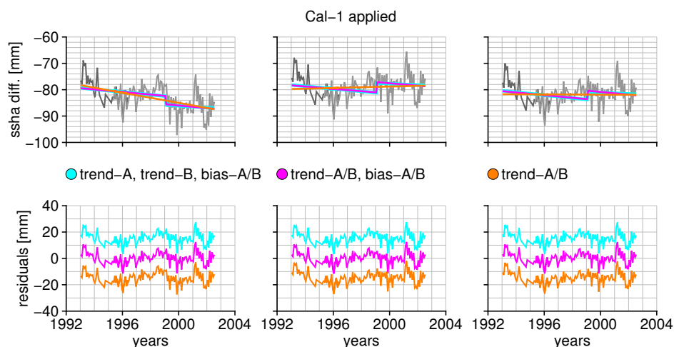
Figure 5.2: Top: time series of sea surface height differences (TOPEX-ERS1&2) for the bm4 (left), CSR (middle) and the CLS (right) SSB models for which cal-1 is applied, together with three models fitted to the data. Bottom: residuals after subtracting the models.
