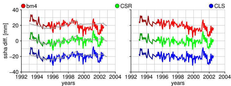
Figure 5.1: Global mean sea surface height differences from crossovers (TOPEX-ERS1&2) for three different SSB models. The darker shading indicates the ERS1 crossovers. Left: Cal-1 is applied and the cal-1 correction is plotted in grey. Right: Cal-1 is not applied.
