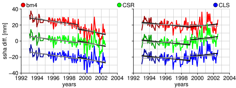
Figure 5.4: Right: Averaged crossover sea-level differences between TOPEX and ERS1&2 over the southern hemisphere. Left: Averaged sea-level differences over the northern hemisphere. Cal-1 is in all cases unapplied.
