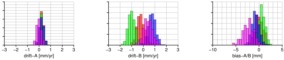
Figure 5.13: Histograms of the TOPEX-A&B drifts and intramission bias for the four averaging methods based on model 3 with the CSR SSB correction applied. Cal-1 is applied to TOPEX-A&B.
