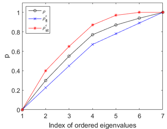
FIG. 3. Majorization curves of the state \rho compared to its steepest and flattest states \rho_{st}^\epsilon and \rho_{fl}^\epsilon , as shown in Figs. 2(a) and 2(b). Any other state \rho' \in \mathcal{B}^\varepsilon(\rho) will have a majorization curve that lies between the red (with “*” markers) and blue (with “x” markers) curves.
