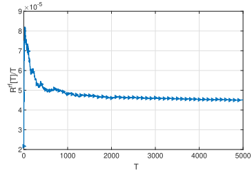
FIGURE 3. Dynamic regret in RF space.
