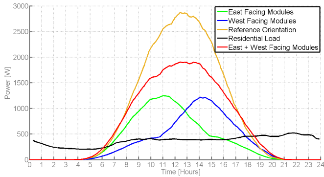
Fig. 10. Power for Optimised Orientation in Spring
