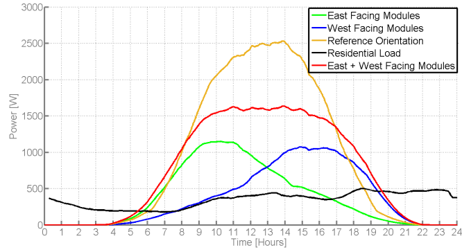
Fig. 11. Power for Optimised Orientation in Summer
