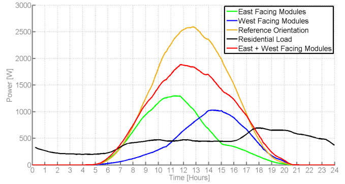
Fig. 12. Power for Optimised Orientation in Autumn
