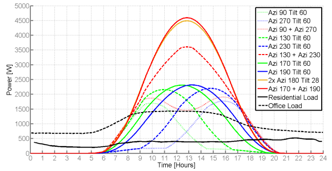
Fig. 4. Power for Varying Azimuth in Spring
