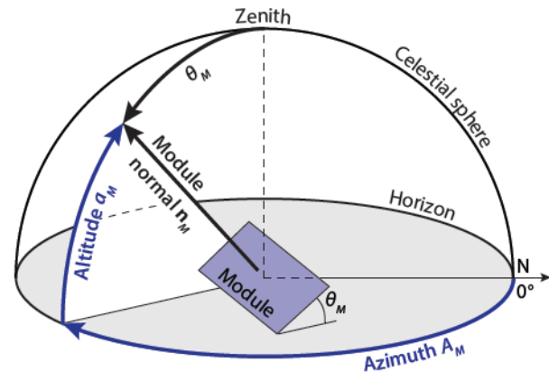
Fig. 1. Angles used in Defining Module Orientation
