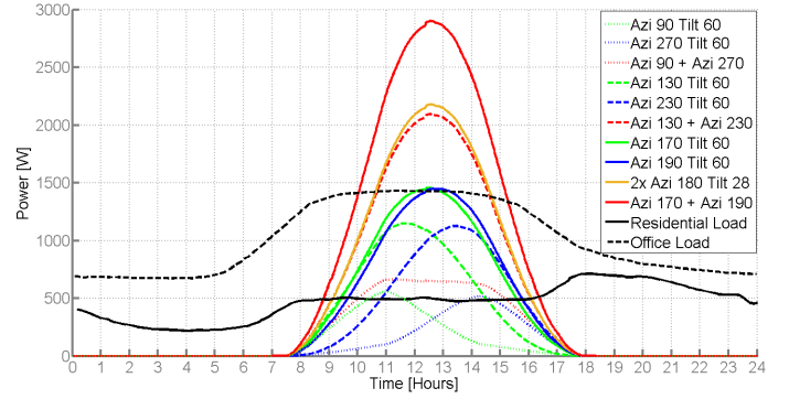
Fig. 2. Power for Varying Azimuth in Winter
