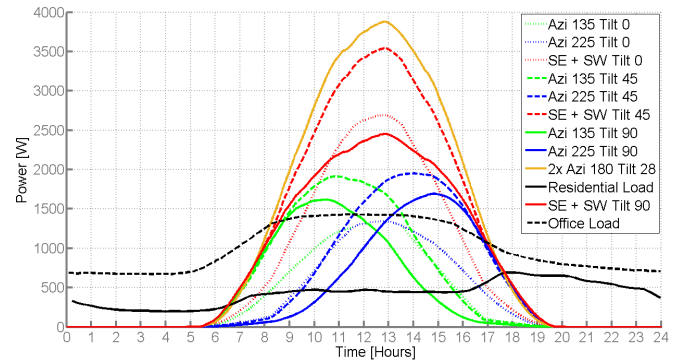
Fig. 9. Power for Varying Tilt in Autumn
