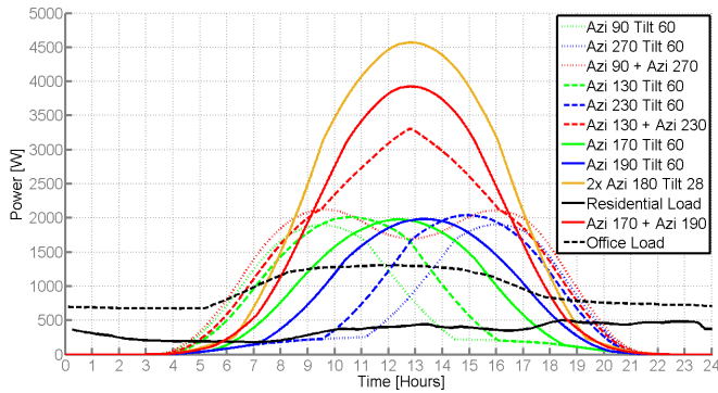
Fig. 6. Power for Varying Azimuth in Summer
