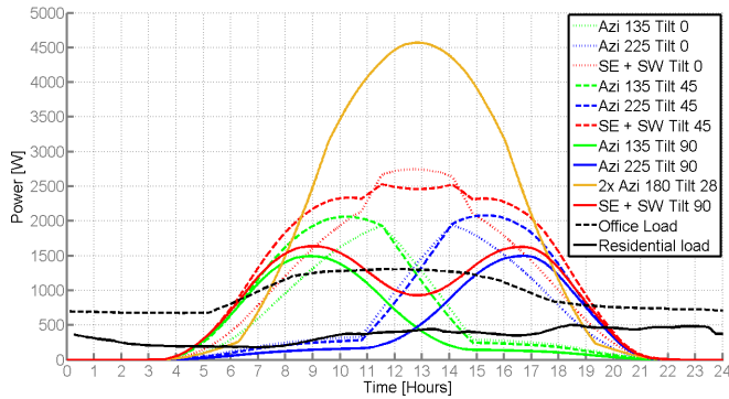
Fig. 7. Power for Varying Tilt in Summer
