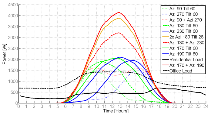
Fig. 8. Power for Varying Azimuth in Autumn
