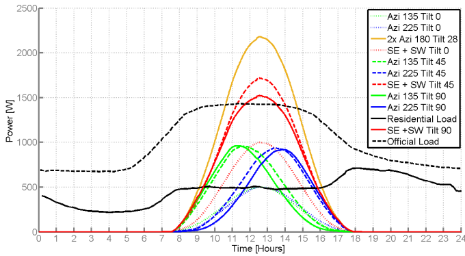
Fig. 3. Power for Varying Tilt in Winter
