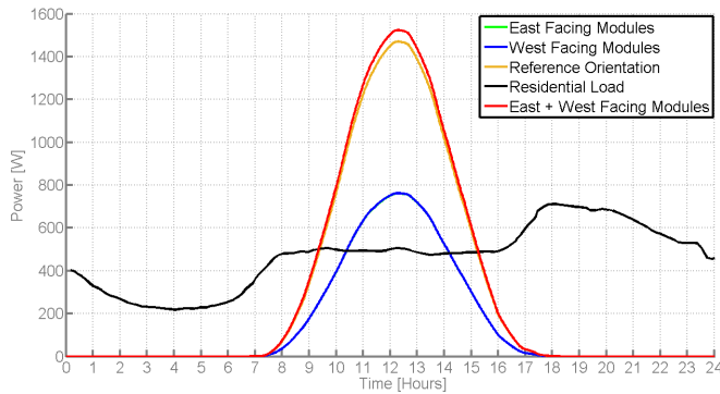
Fig. 13. Power for Optimised Orientation in Winter
