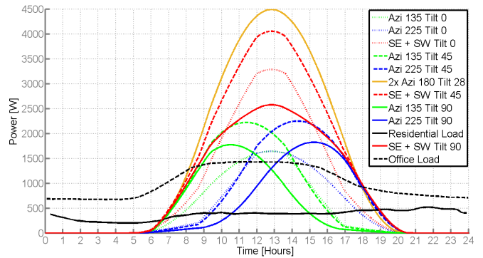
Fig. 5. Power for Varying Tilt in Spring
