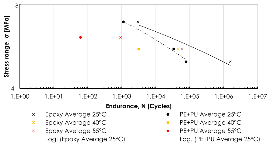
Fig. 15. Endurance of SRR at 25 °C, 40 °C and 55 °C for epoxy and UPE + PU resin systems.
