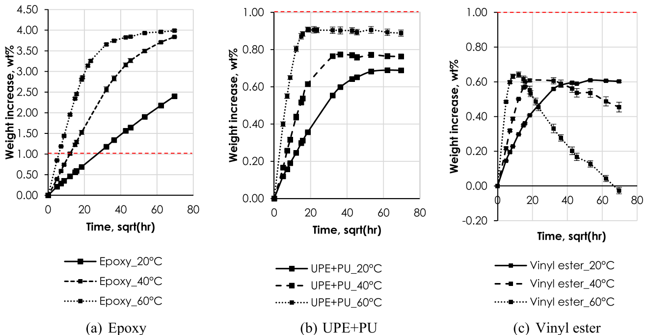
Fig. 17. Weight change of pure resins versus square root of water immersion time, square( t ) for temperatures varying from 20 °C to 60 °C (red dashed line included at 1.0% as a reference in all three graphs).
