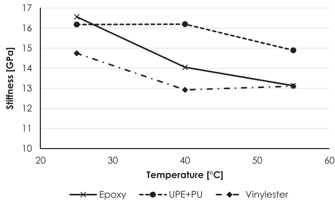
Fig. 9. Average stiffness variation under various temperatures.
