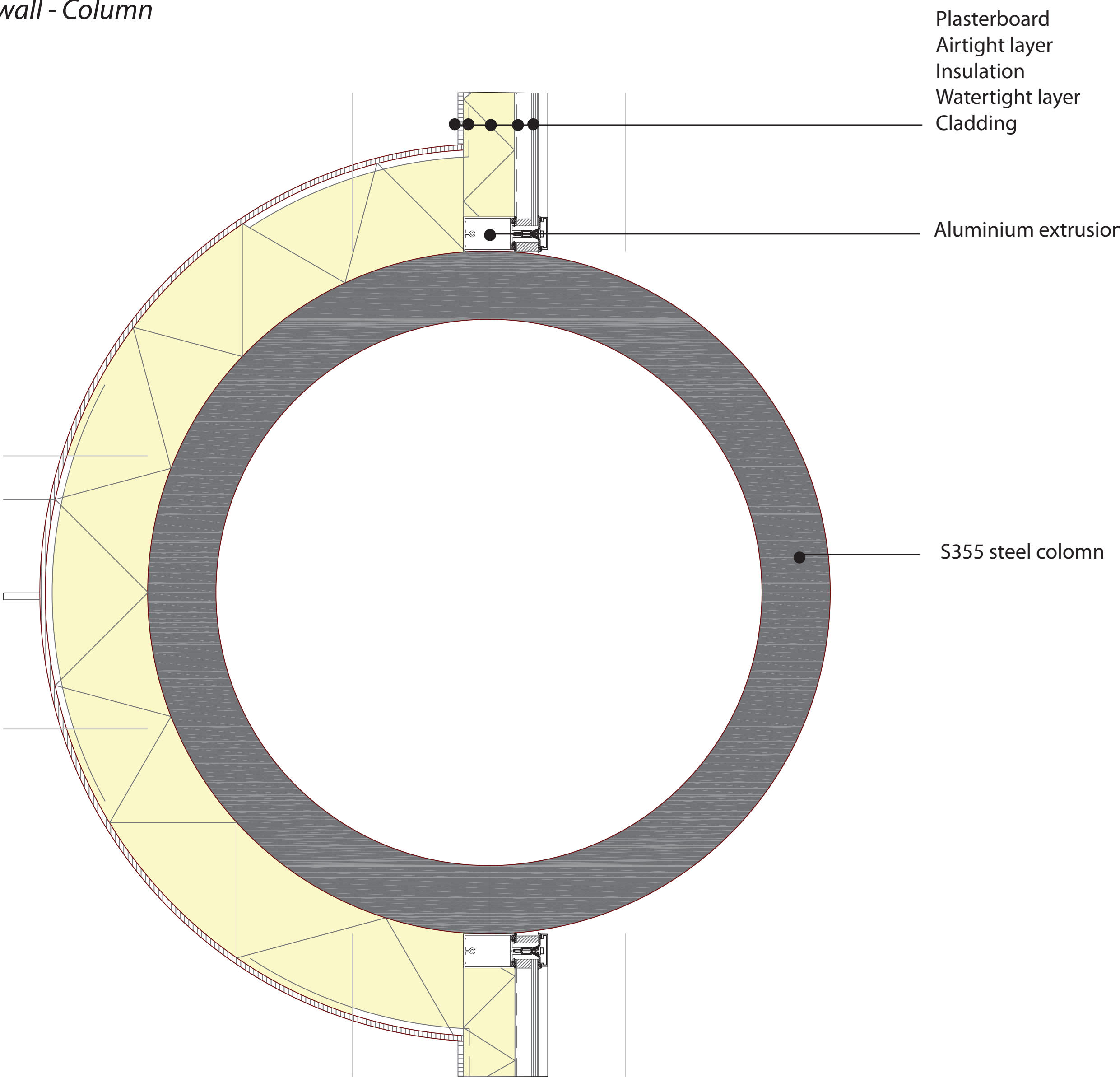
Detail 5 Curtain wall - Column
