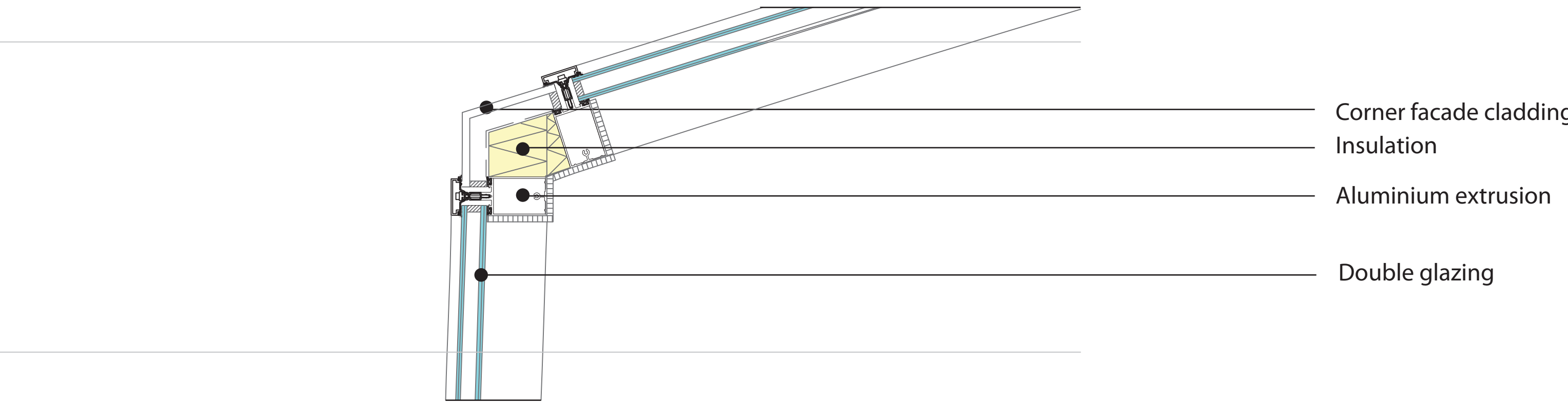
Detail 2 Glass - ETFE
