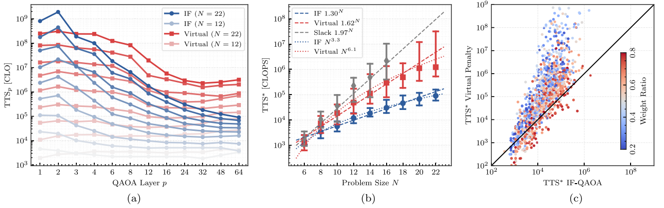
FIG. 5. (a) shows the median TTS for all problem instances in various color shades with increasing QAOA layer count p . As apparent, IF-QAOA starts with higher TTS than the baseline approach, but starts improving upon it starting with p \geq 3 . (b) shows the optimal TTS* depending on the problem size. The dashed line shows the logarithmic regression, with the fitted bases displayed in the legend. (c) shows a scatter plot of all 9 \times 128 = 1152 problem instances comparing TTS* of IF-QAOA against the virtual penalty. In 82% of the test cases, IF-QAOA arrives at a solution faster. The color shading of the scatter plots indicates the weight ratio W/\sum_i w_i of the knapsack instance.
