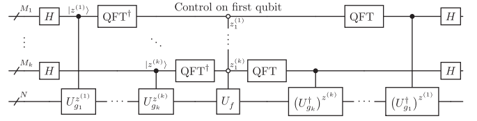
FIG. 3. Multiconstraint cost function subroutine. The first qubits of the QPE registers control the application of the cost operator.
