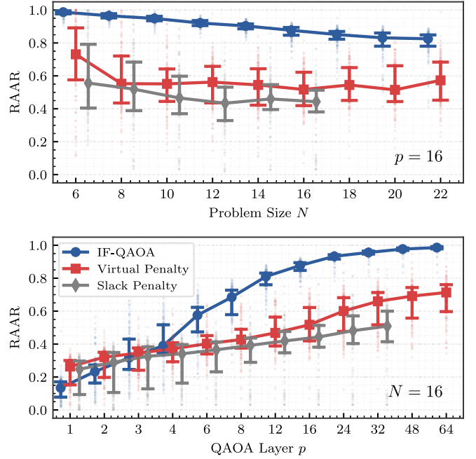
FIG. 4. The solution quality measured as RAAR displayed for a selection of results. The top plot shows RAAR depending on problem size N for fixed QAOA layer depth p = 16 , and the bottom plot shows RAAR w.r.t. p at N = 16 . Error bars indicate the 50% percentile interval.
