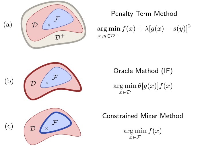
FIG. 1. Showcasing the search spaces of the various optimization strategies. In (a), the search space is enlarged to \mathcal{D}^+ through slack variables in the penalty term. In (b), the search space is exactly the space of the originally defined problem, and in (c), the search space is effectively reduced to the feasible subspace. The shapes of the domains are exemplary.
