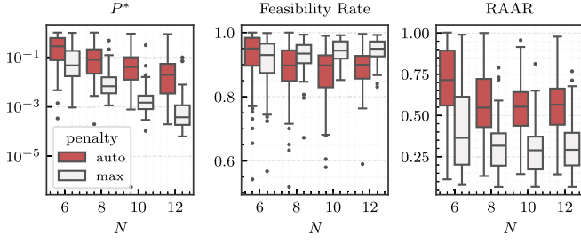
FIG. 9. Probability of sampling the optimal solution, feasibility rate \sum_{x \in \mathcal{F}} |\langle x | \psi \rangle|^2 , and RAAR at p = 16 for different problem sizes w.r.t. penalty settings, where auto refers to Eq. (24).
