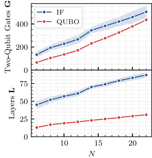
FIG. 10. Circuit resources of IF-QAOA and QUBO-QAOA for the considered knapsack instances for problem size N .
