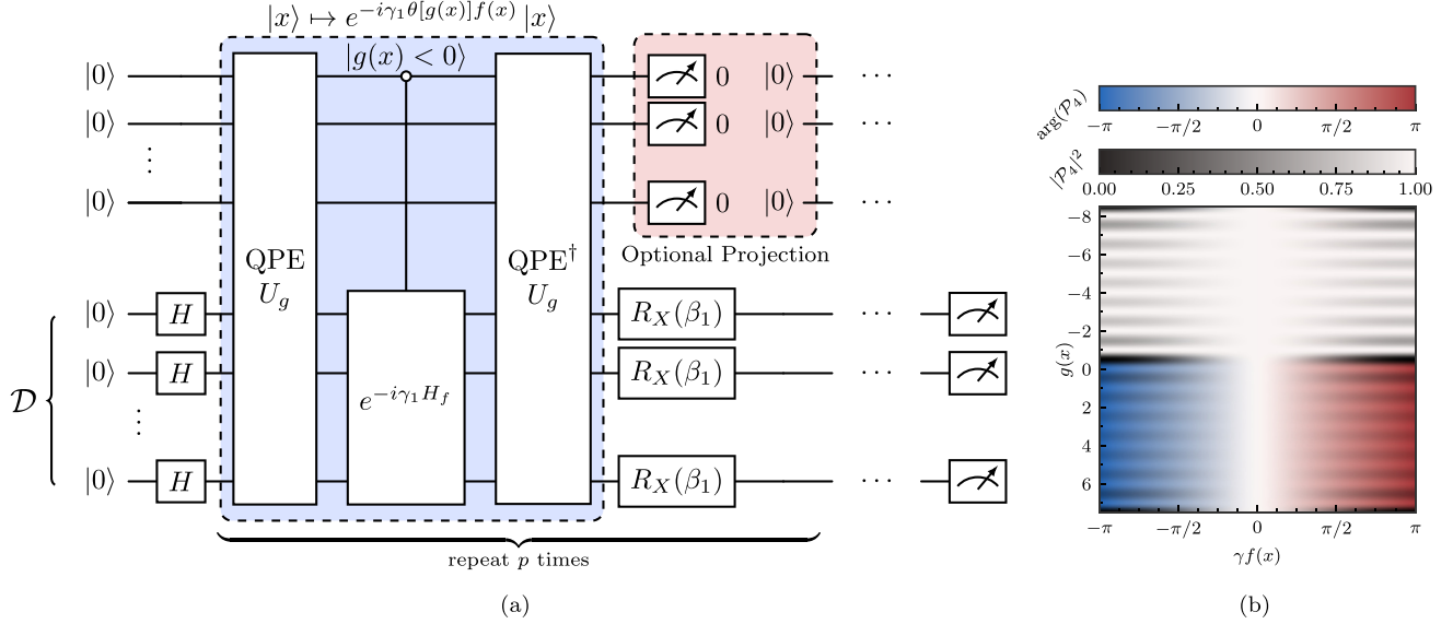
FIG. 2. (a) Shows the IF-QAOA circuit. The cost layer consists of the QPE, evaluating whether constraint g has been satisfied, and a controlled application of the cost Hamiltonian based on the indicator qubit. The projective measurement on the QPE register is only required when g is not resolvable by the QPE register. (b) IF-QAOA circuit presents the projection factor \mathcal{P} , defined in Eq. (21), in the approximate application of the indicator function, when g is not resolvable by the QPE register, here for M = 4 . The shading of the plot shows the probability of successful projective measurements. Clearly, when g is an integer, this probability is always one. The hue indicates the applied phase to the compute register, showing that the application only happens for g(x) \geq 0 .
