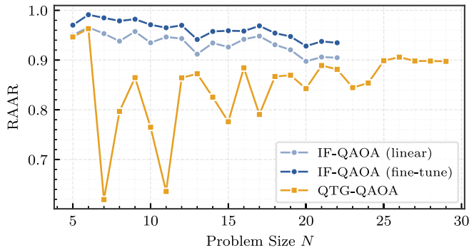
FIG. 7. RAAR of IF-QAOA (for p , see Table I) compared to QTG-QAOA at p = 1 . IF-QAOA is separated between two results: linear refers to optimizing just the rates of the linear schedule. Fine tune refers to running 100 L-BFGS iterations on all parameters, starting with the optimized linear schedule. Results for QTG-QAOA and problem instances are taken from Ref. [24].
