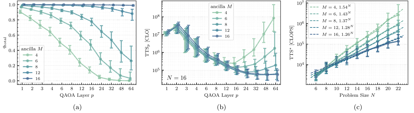
FIG. 8. The success probability q_{\text{total}} for different M is depicted in (a). (b) shows the TTS w.r.t. the QAOA repetitions for problem size N = 16 . Clearly, fewer ancillary variables lead to a sudden increase in TTS after p \approx 16 due to vanishing success probability. TTS is relatively similar for shorter QAOA circuits. \text{TTS}^* scaling is shown in (c), with more ancillary variables leading to more favorable scaling. However, we also see that the scaling saturates and is very comparable for M \geq 12 .
