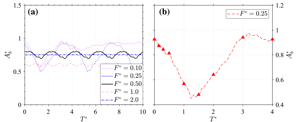
Fig. 17 a Phase-averaged variation of the backflow area with increasing frequency at \alpha = 22^\circ . b Zoomed-in view of the phase-averaged backflow area in one actuation period at F^* = 0.25 . The instants shown in Fig. 18 are indicated by triangles
