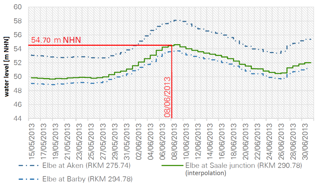
Figure 3. Graphs with water levels over time of the Elbe and Saale near Aken and Barby. Water level at Elbe and Saale junction, RKM 290.8, is NHN+54.7 m (Drews, 2017; Grubert, 2013)
