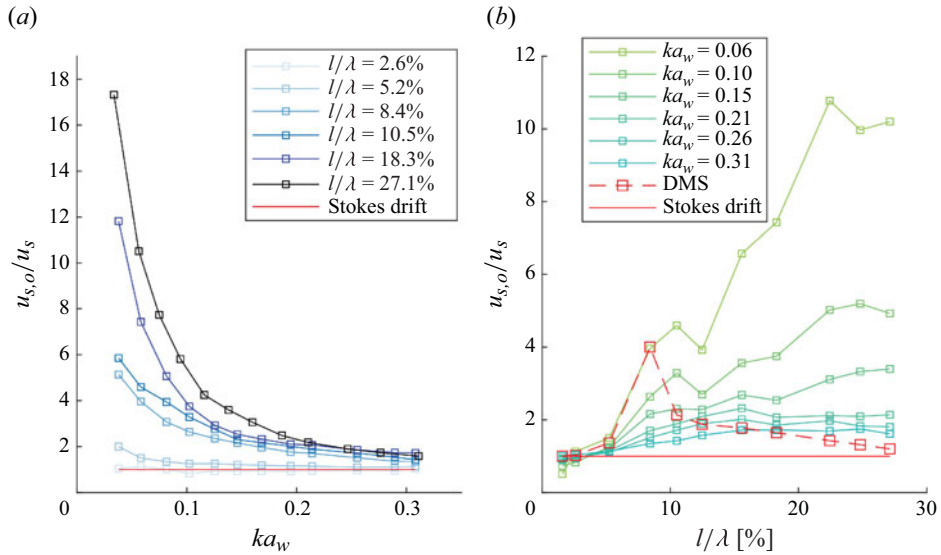
Figure 11. Stokes drift-normalised Stokes object drift (a) as a function of wave steepness for different relative object sizes and (b) as a function of relative size for different values of wave steepness. An idealised Lagrangian particle with zero enhanced drift would have u_{s,o}/u_s = 1 . The red dashed line with red square labelled DMS represents the diffraction-modified Stokes drift given by (3.3). As the diffraction-modified Stokes drift for a certain object size does not change with wave steepness (we use a linear ‘BEM’ model to solve (3.3), and (3.3) is a second-order accurate quantity), it is shown as a single line in panel (b).
