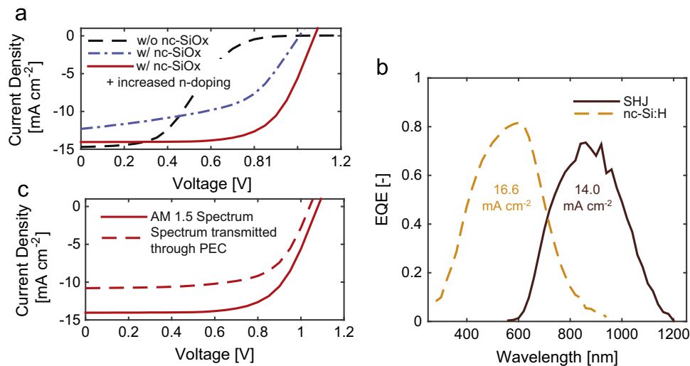
Fig. 7. Optimization of nc-Si:H/SHJ hybrid tandem cell. (a) J - V curve of the hybrid solar cell with different TR configurations. (b) EQE curves of the optimized hybrid solar cell. (c) Shifting of the J - V curve of the hybrid cell when a standard PEC is used as a filter to only allow the light that would hit the hybrid cell if it were integrated into a monolithic PEC/PV structure.
