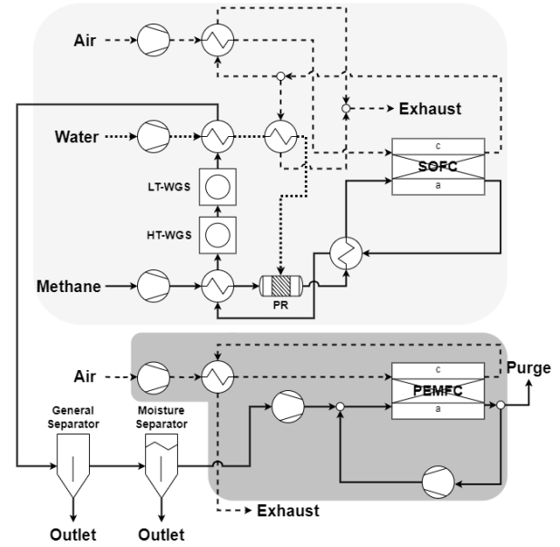
Figure 1: SOFC-PEMFC combined cycle system layout
