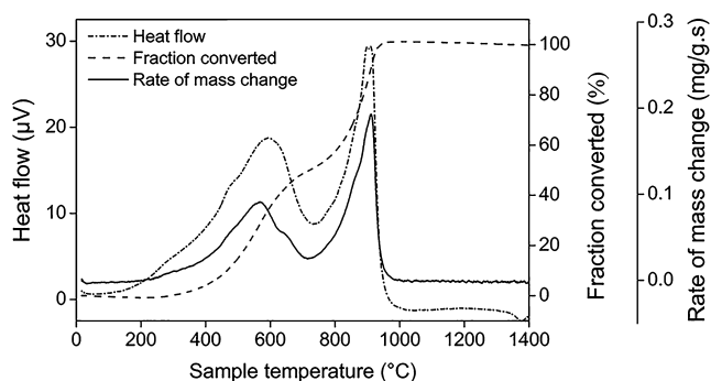
FIGURE 4 Oxidation kinetics of \text{Ti}_2\text{AlC} powder in air at 4^\circ\text{C}/\text{min} : heat flow, fraction converted, and rate of mass change (recorded mass change differentiated) vs temperature
