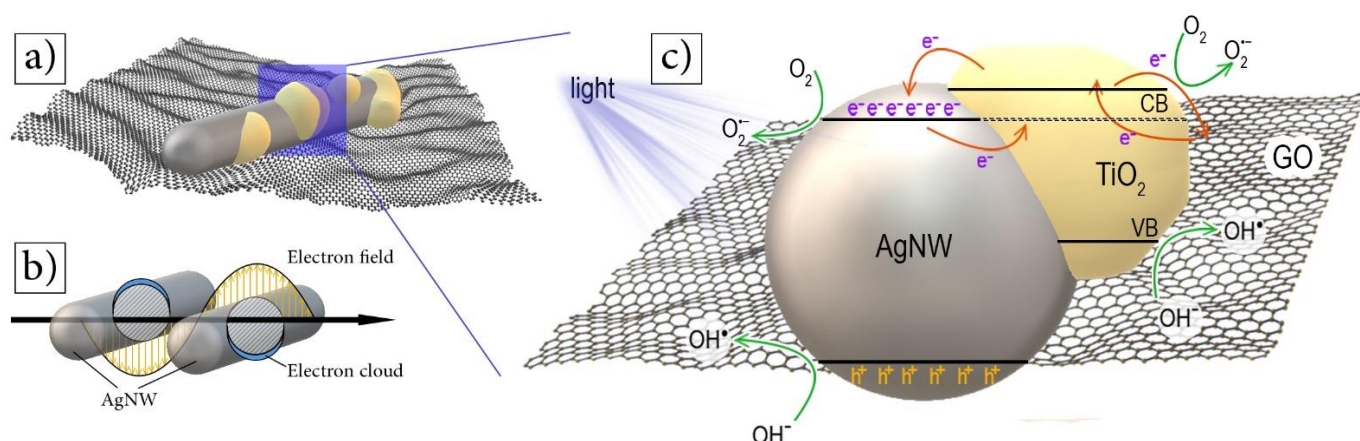
Figure 11. Schematic diagrams of (a) AgNW/ \text{TiO}_2 /GO nanocomposite structure, (b) localized SPR of AgNWs when irradiated with visible or UV light, and (c) photocatalytic mechanism of AgNW/ \text{TiO}_2 /GO nanocomposites.
