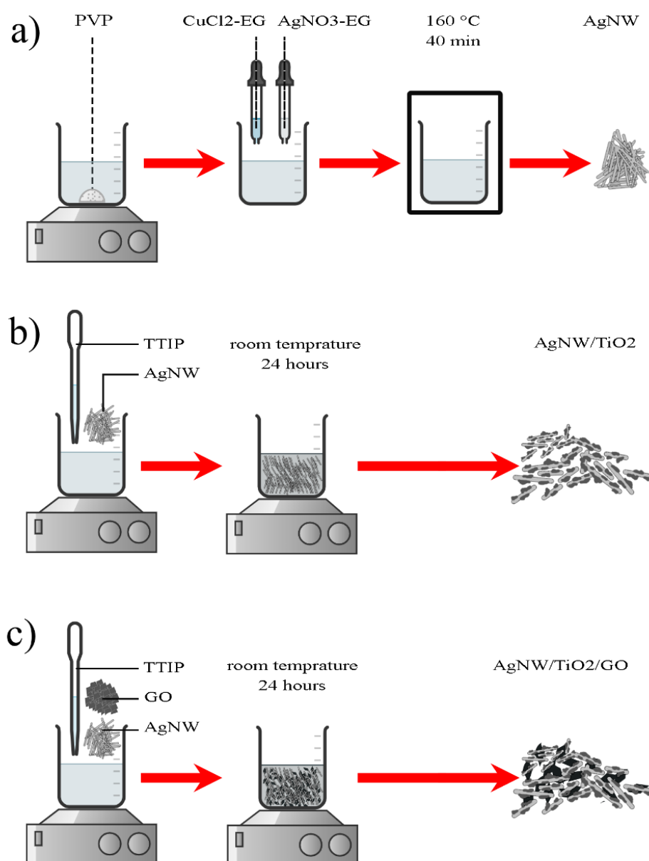
Figure 1. A schematic diagram describing the synthesis process of (a) AgNW, (b) \text{AgNW}/\text{TiO}_2 , and (c) \text{AgNW}/\text{TiO}_2/\text{GO} samples.
