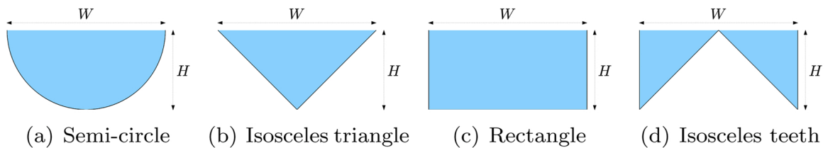
Figure 11. Idealized initial shapes of the corrosion pit in the two-dimensional pit test example. The blue area is the electrolyte domain \Omega_E , the black line is the interface \Gamma_{\text{I}} , and the solid domain is not shown.
