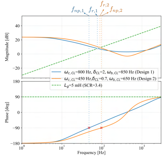
Fig. 9. Bode plots of the Z_{dd}(s) with three different \omega_{b,CL} .
