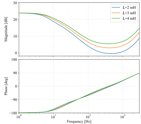
Fig. 10. Bode plots of the Z_{dd}(s) with three different power filter inductance L .
