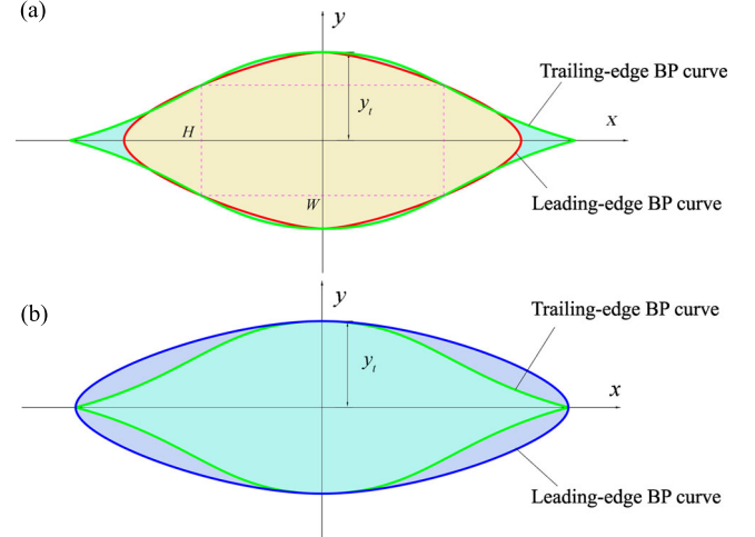
Figure 3 Leading-edge and trailing-edge BP curve geometry. (a) Equal clearance; (b) equal AR
