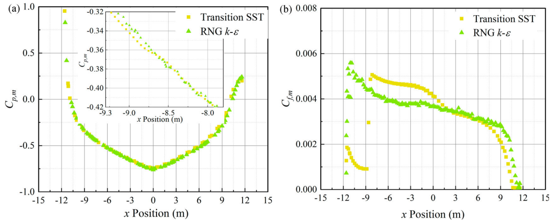
Figure 13 Comparison between transition SST and RNG k-\varepsilon models. (a) C_{p,m} ; (b) C_{f,m}
