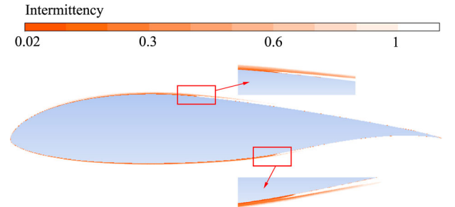
Figure 8 Intermittency contours at R_e = 4 \times 10^6
