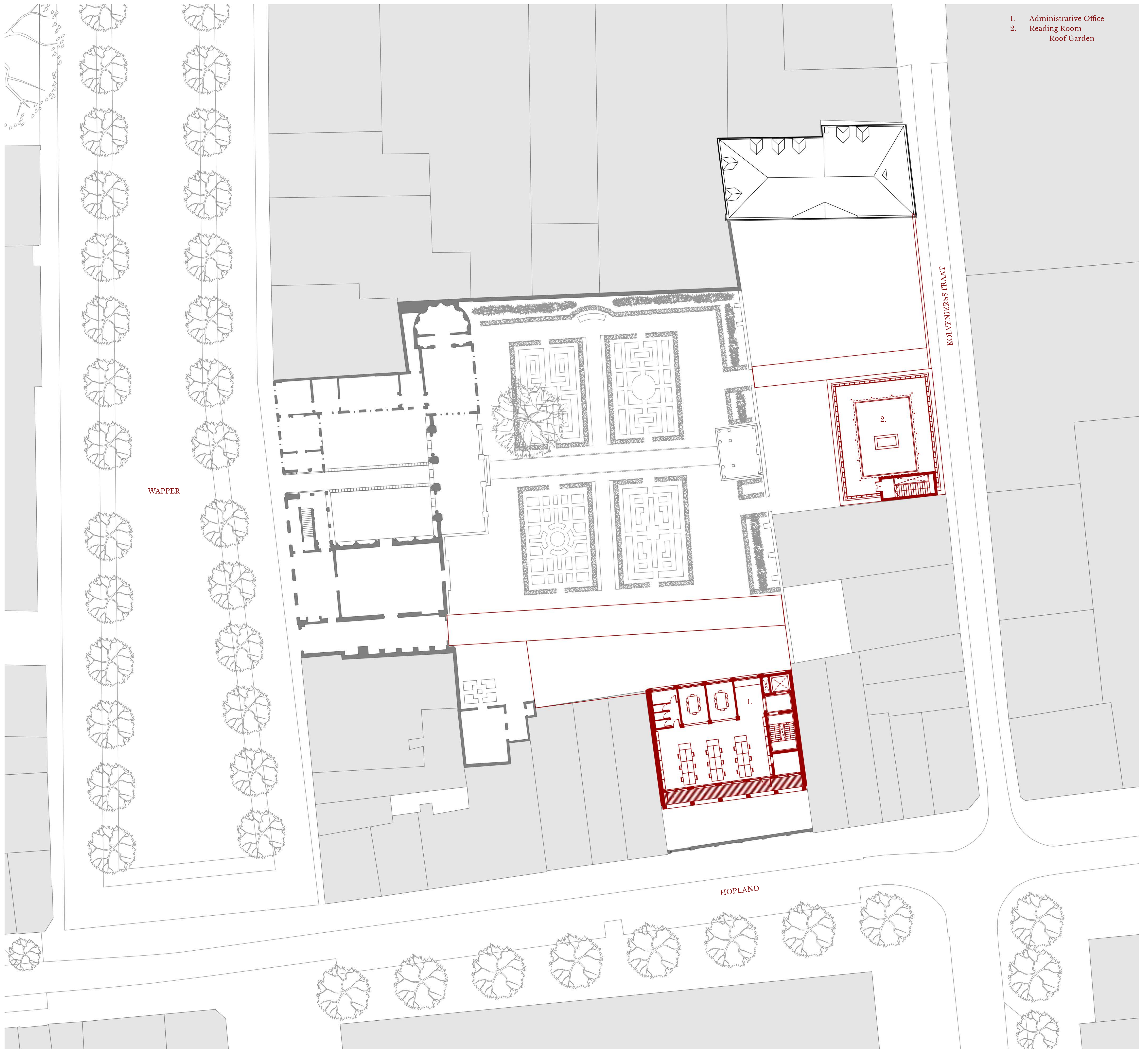
Third Floor Plan - 1:200
