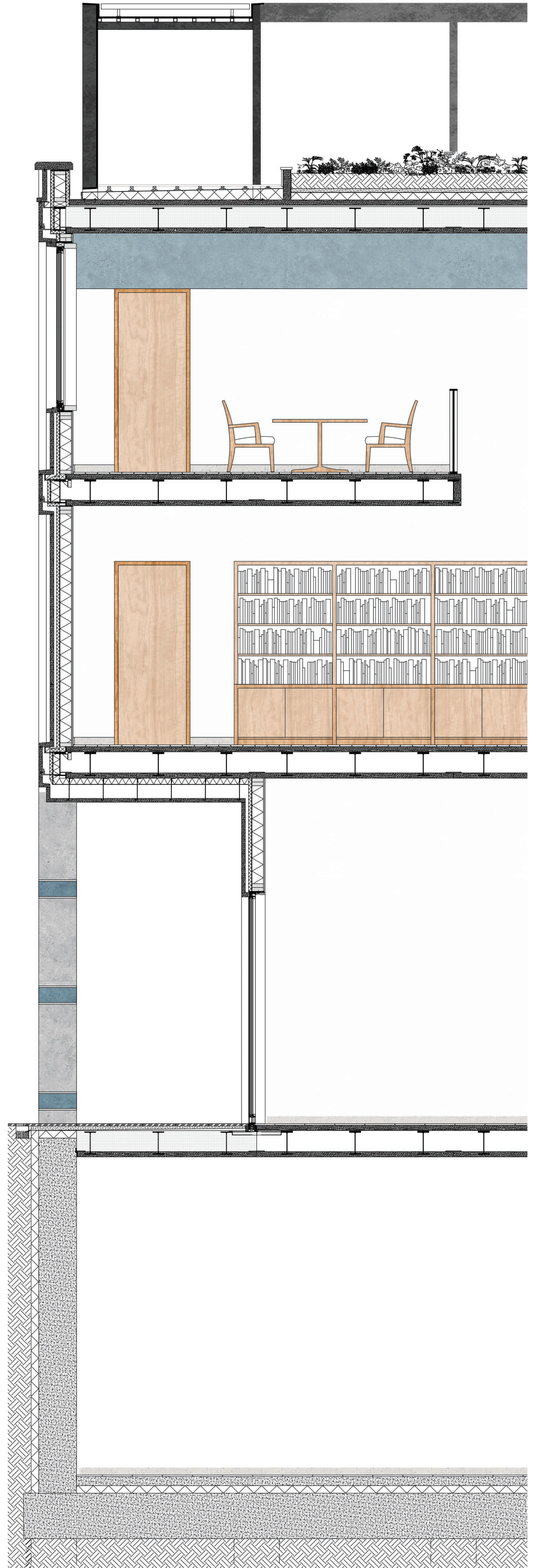
Reading Room Section - 1:20
