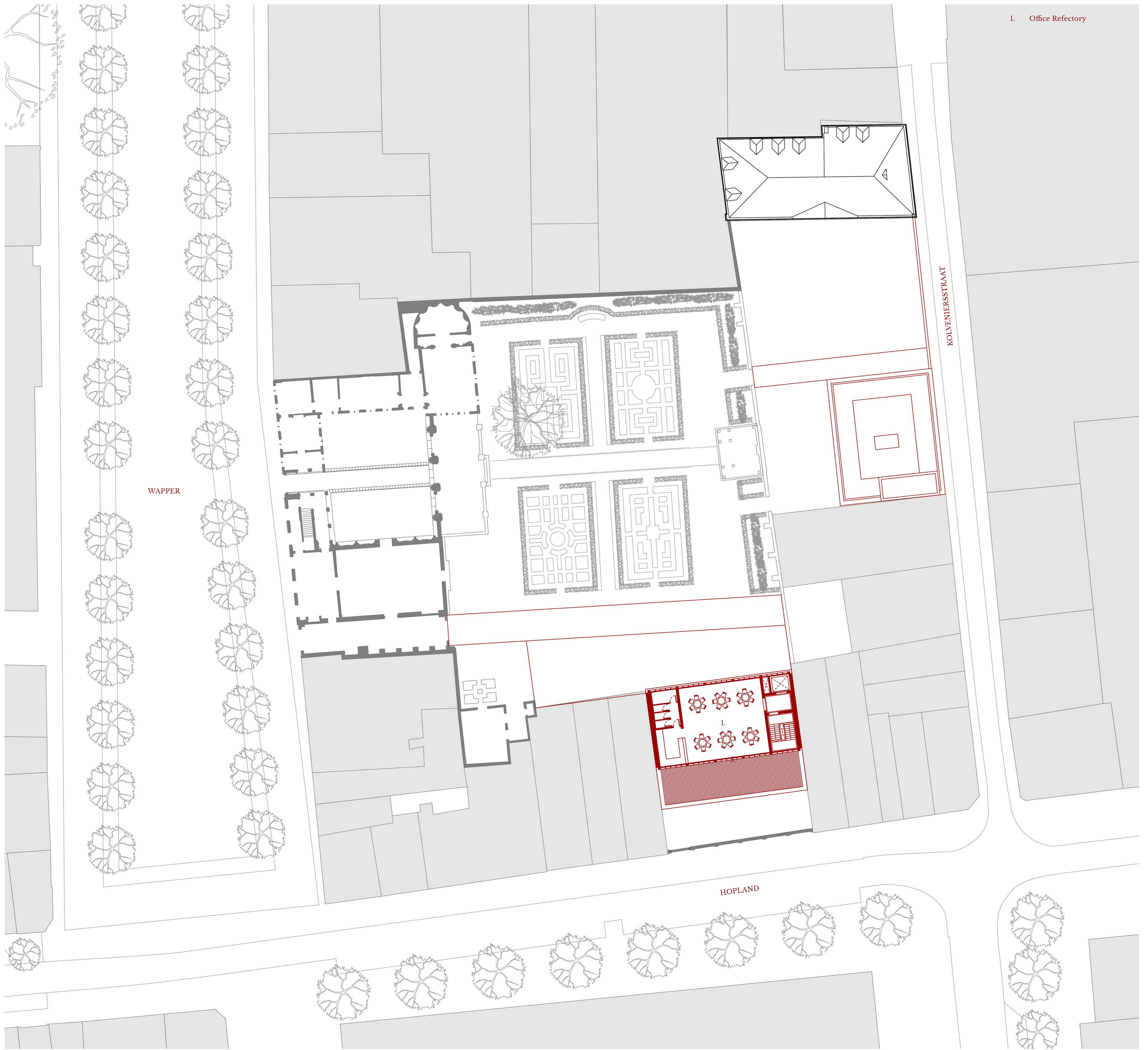
Fifth Floor Plan - 1:200
