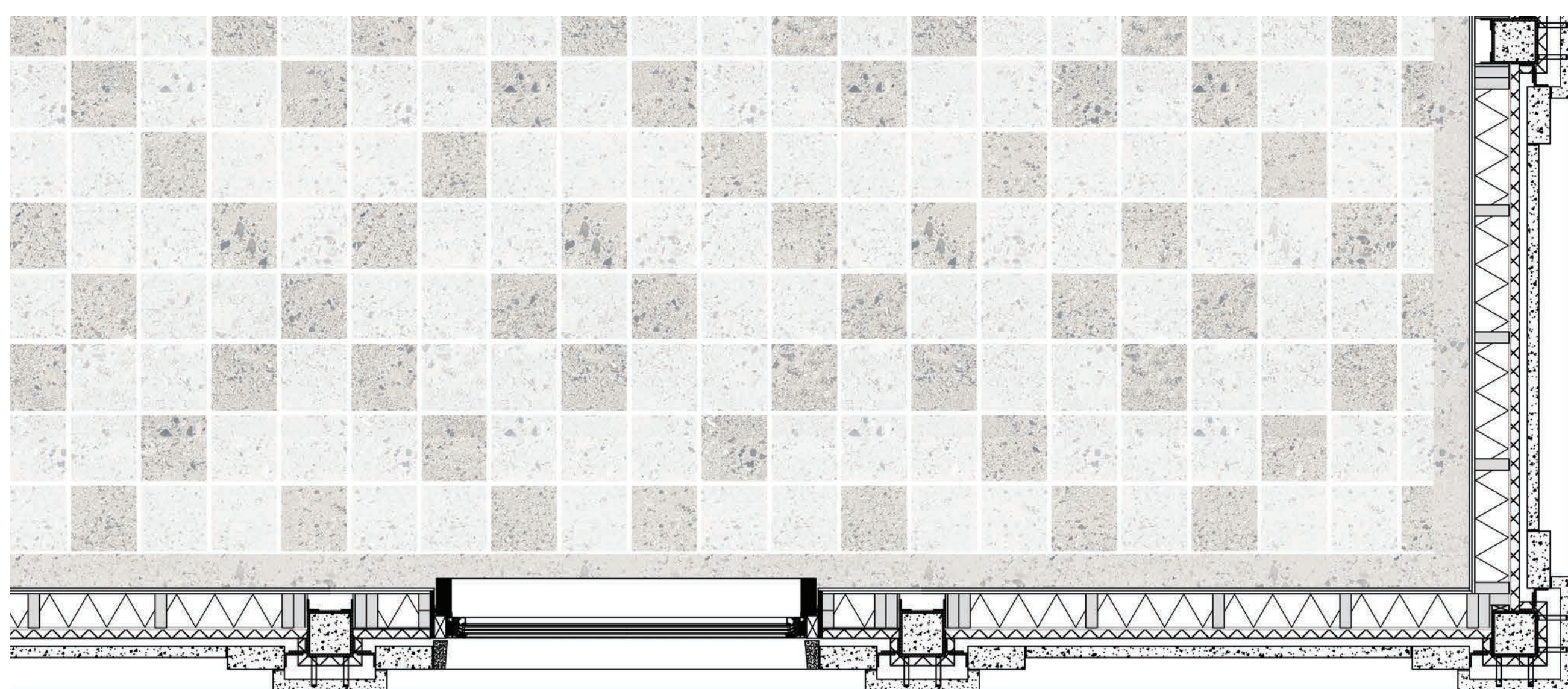
Reading Room Plan - 1:20
