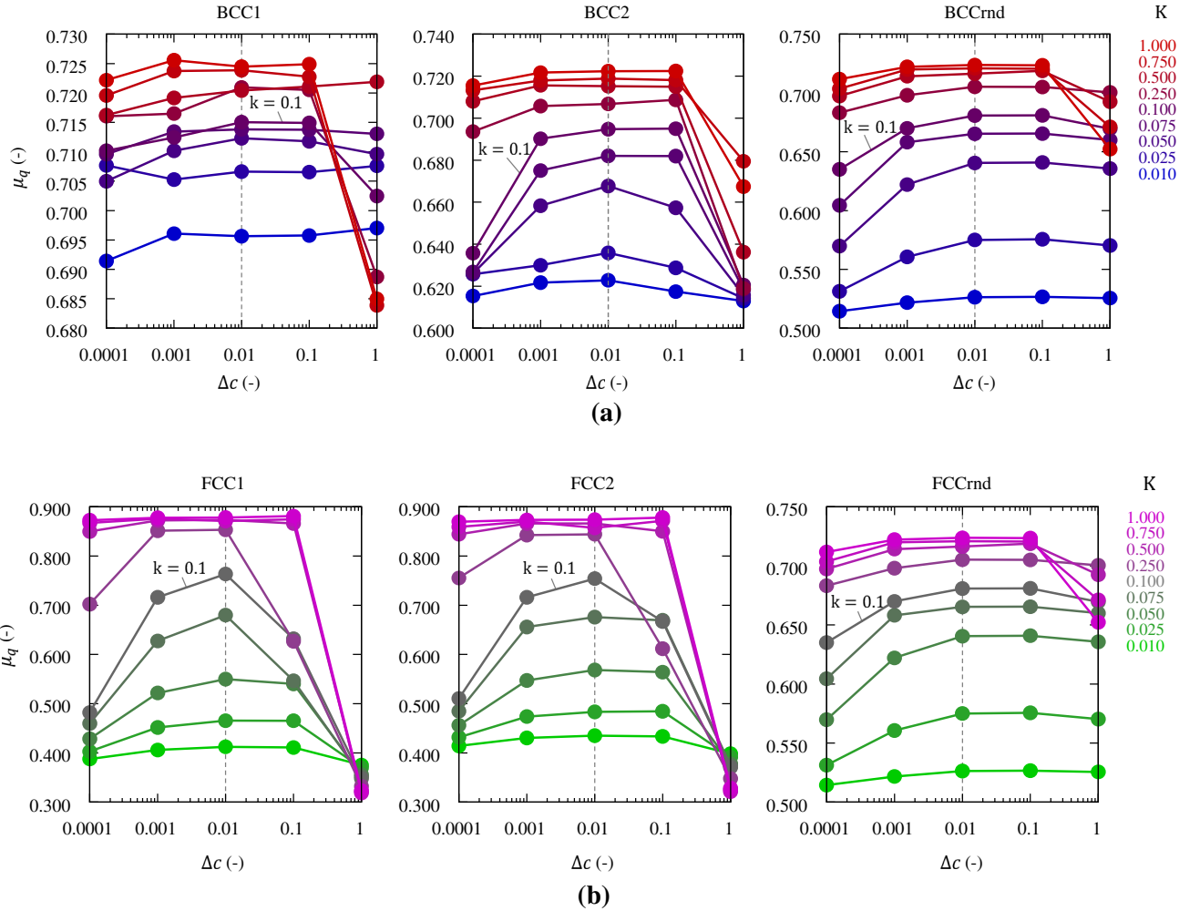
Fig. 11—Value of \mu_q obtained for k = 0.01, 0.025, 0.050, 0.075, 0.1, 0.25, 0.50, 0.75, 1 and \Delta c = 0.0001, 0.001, 0.01, 0.1, 1 after 50 optimization steps for (a) BCC and (b) FCC textures.
