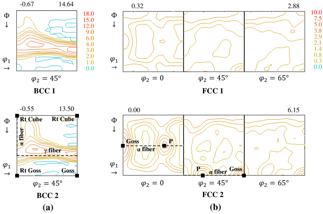
Fig. 2—Selected sections of the ODFs of the initial textures: (a) BCC textures ( \phi_2 = 45 deg section). (b) FCC textures (sections at \phi_2 = 0, 45 and 65 deg). On top, the minimal and maximum values of the ODF are displayed.
