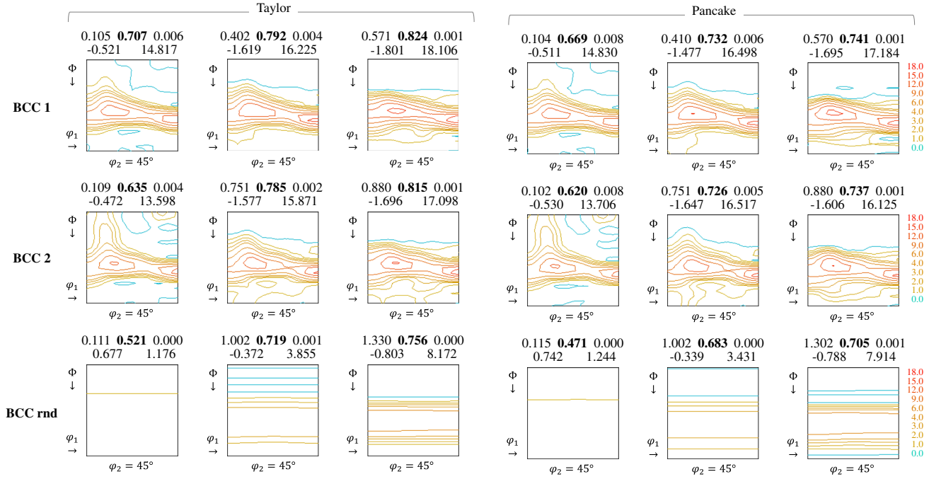
Fig. 8—BCC textures obtained during the optimization process. On top, the variations of the ODF [see (10)], \mu_q (in bold) and \sigma_q , corresponding to each texture, are displayed on the first line and the maximum and minimum values on the second one. For each case, the ODF sections corresponding to three different instants of the optimization are shown: at the beginning of the process, the approximate middle and the end of the process.
