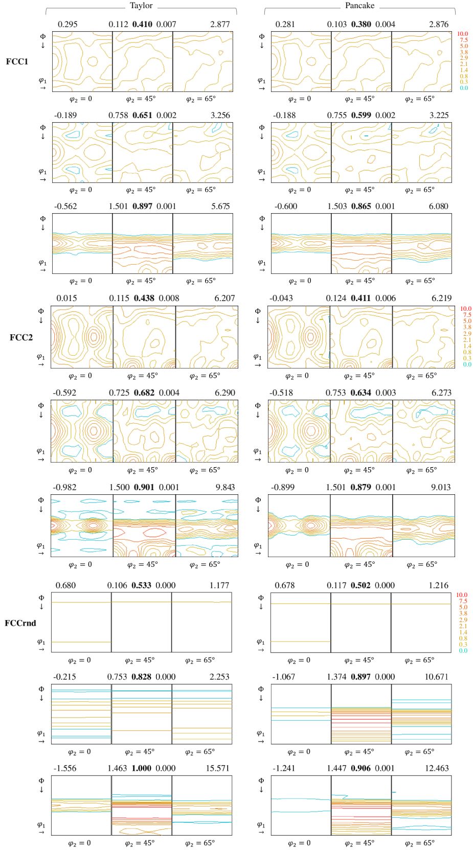
Fig. 9—FCC textures obtained during the optimization process. On top, the variation of the ODF [see equation [10]], \mu_g (in bold) and \sigma_g , corresponding to that texture, as well as the maximum and minimum values. For each case, the ODF sections corresponding to three different instants of the optimization are shown: at the beginning of the process, the approximate middle and the end of the process.
