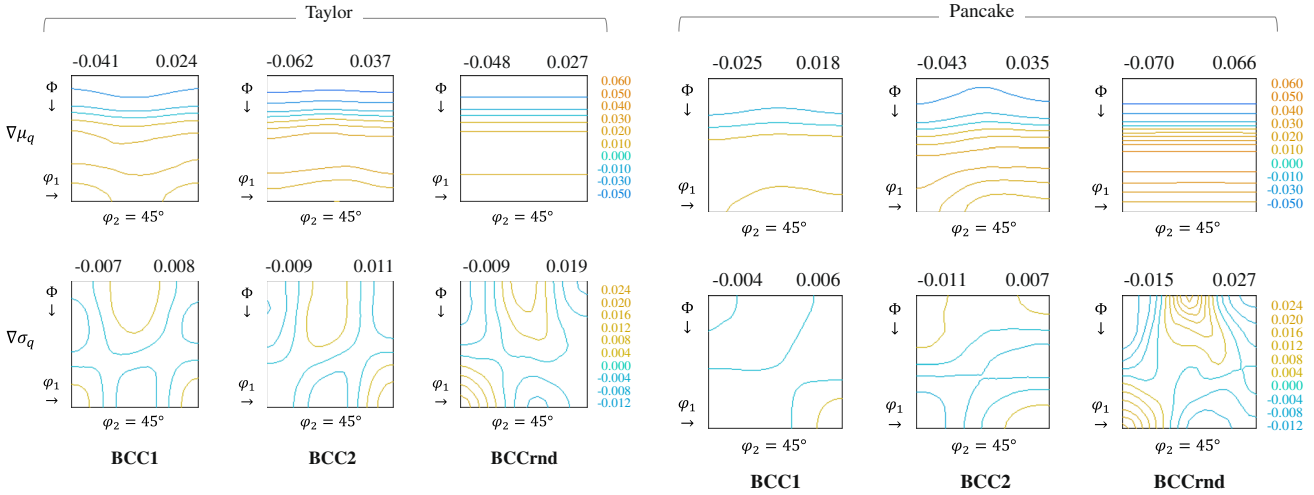
Fig. 5—Initial gradient distribution function of the average q values ( \mu_q ) and their standard deviation ( \sigma_q ) for the textures in Figure 2 using the Taylor and pancake models, calculated using \Delta c = 0.01 . Maximum and minimum values are displayed on top.
