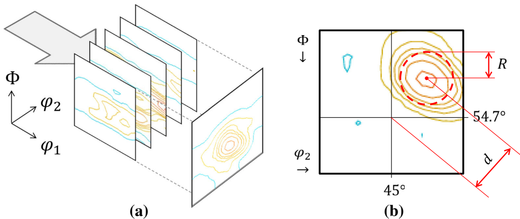
Fig. A1—Schematic diagram of the calculation of fiber textures integrating over \phi_1 (a) and the d and R magnitudes (b), corresponding to the distance to the \gamma fiber at \varphi_2 = 45 deg and \Phi = 54.7 deg and the radius of the fiber texture.
