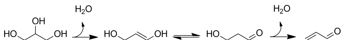
Scheme 15. Acrolein formation mechanism.
