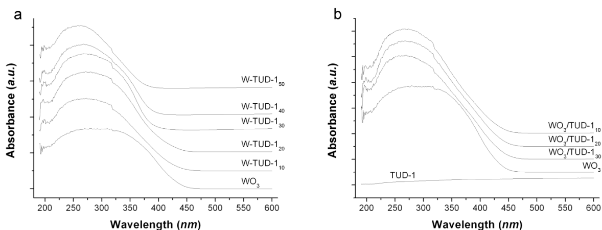
Figure 5. DR UV-Vis spectra of a) W-TUD-1 and b) \text{WO}_3/\text{TUD-1} samples.
