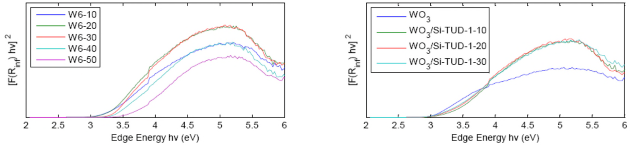
Figure S2. UV-vis DR spectra and Tauc-plots of the W-TUD-1 and WO 3 /TUD-1 materials.
