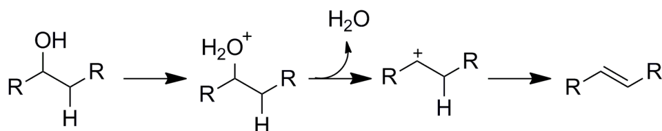
Scheme 1. E 1 mechanism.
