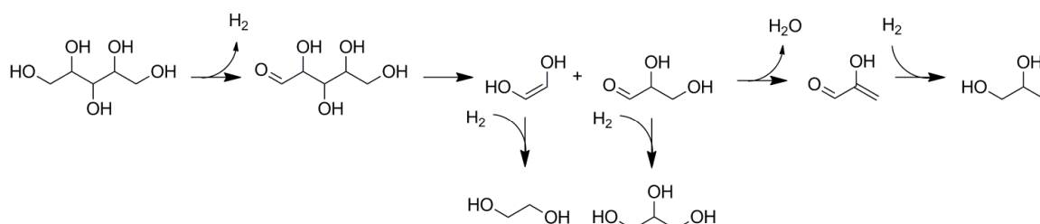
Scheme 21. Xylitol hydrogenolysis under alkaline conditions.
