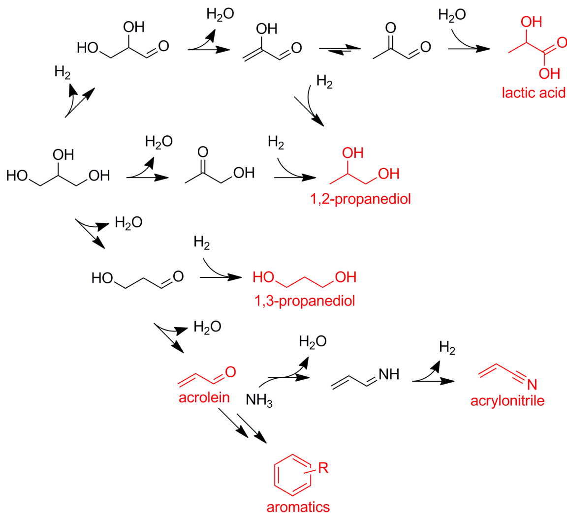
Scheme 8. Dehydrated products from glycerol.
