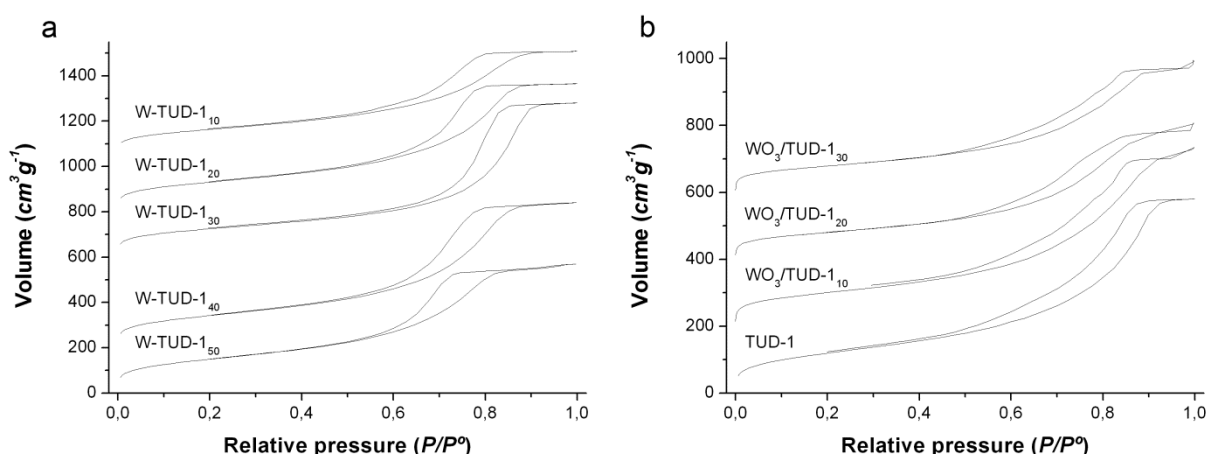
Figure 1. Nitrogen physisorption isotherms for a) W-TUD-1 and b) WO 3 /TUD-1 samples and pore size distribution for c) W-TUD-1 and d) WO 3 /TUD-1 samples.
