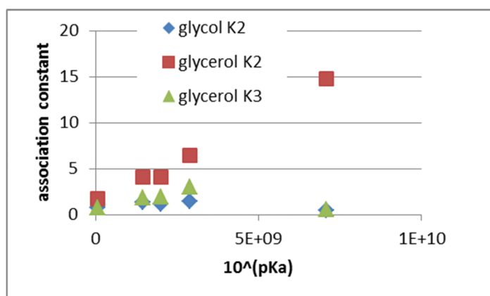
Figure 5. Exemplifying differences in K values and pK_a 's from Table 2. (acidic boronic acids on the left, boric acid on right (forming most of the borate ester).
