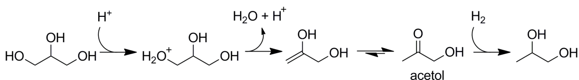
Scheme 11. 12PD formation from glycerol under acidic conditions.
