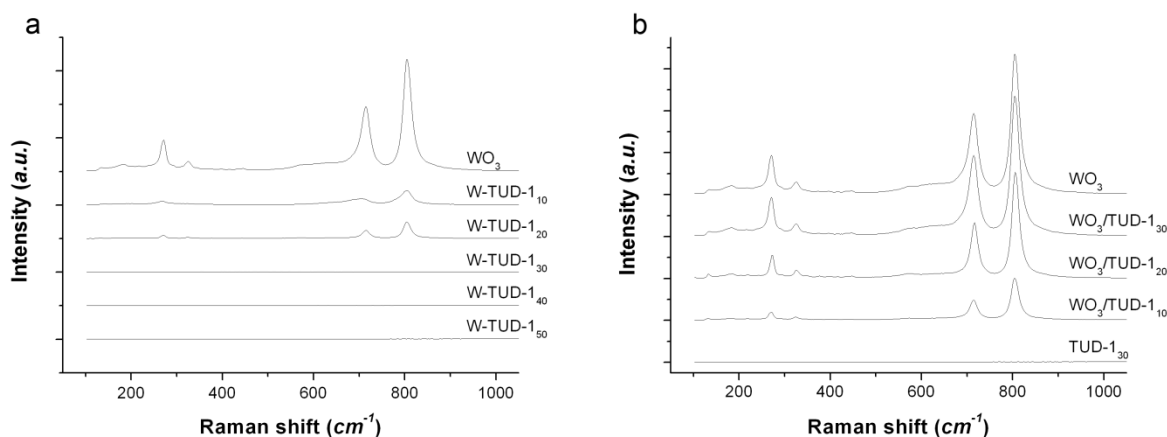
Figure 3. Raman spectra of a) W-TUD-1 and b) WO 3 /TUD-1 samples.
