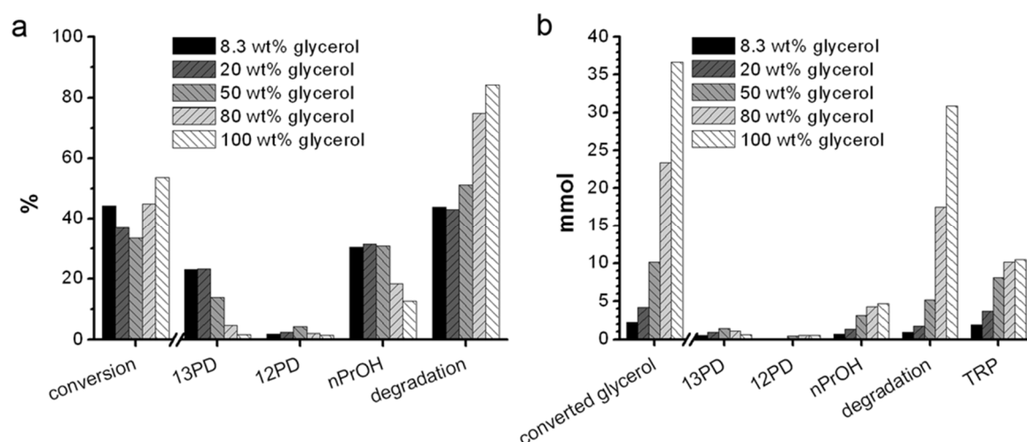
Figure 5. Reduction of concentrated aqueous glycerol solutions. Reaction conditions: 97.5 mg \text{Pt}/\text{Al}_2\text{O}_3 ; 3.5 mM silicotungstic acid; 40 bar \text{H}_2 ; 200 ^{\circ}\text{C} ; 18 h; 800 rpm.
