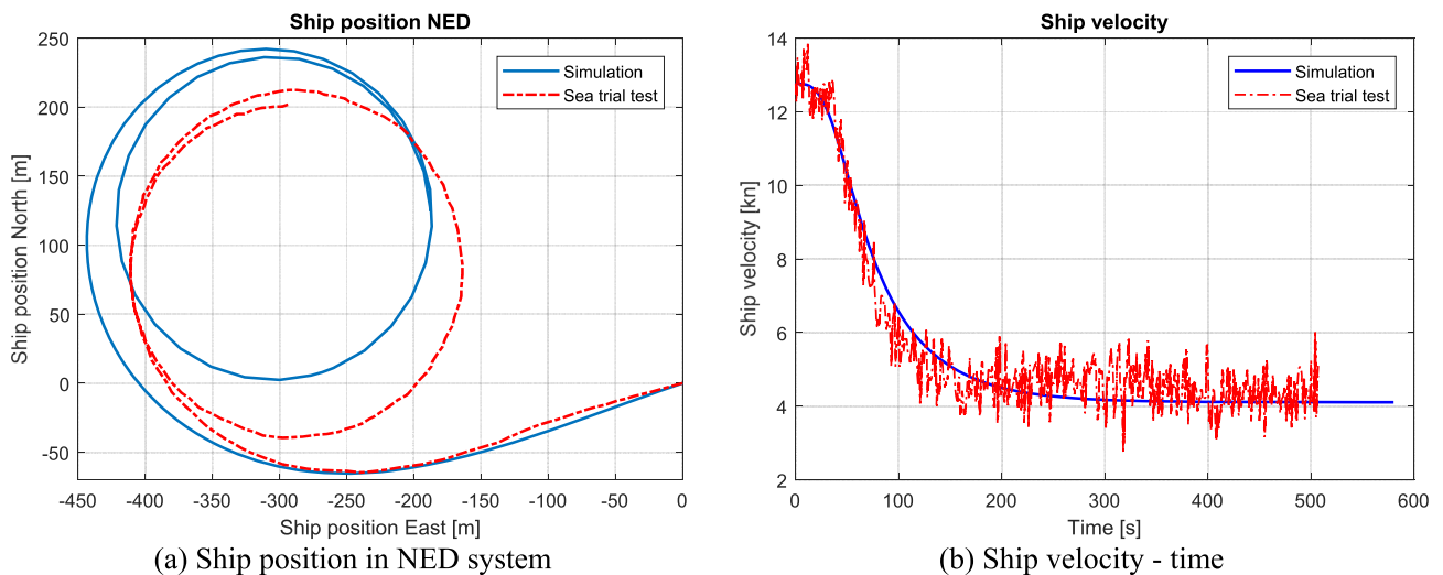
Fig. 7. Validation results of turning circle trial (Starboard with rudder angle: 35 deg.).
