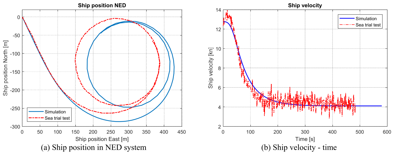
Fig. 6. Validation results of turning circle trial (Portside with rudder angle: 35 deg.).
