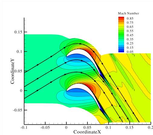
Figure 9: Mach number contours around the t106c nozzle guide vane
