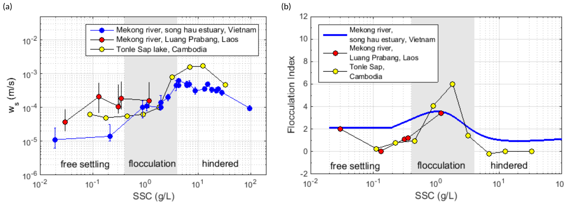
Fig. 5. Sediment properties in the Mekong Land to Ocean Continuum: (a) Variation of settling velocity with SSC measured directly with SCAF instrument and (b) Variation of the flocculation index with SSC.
