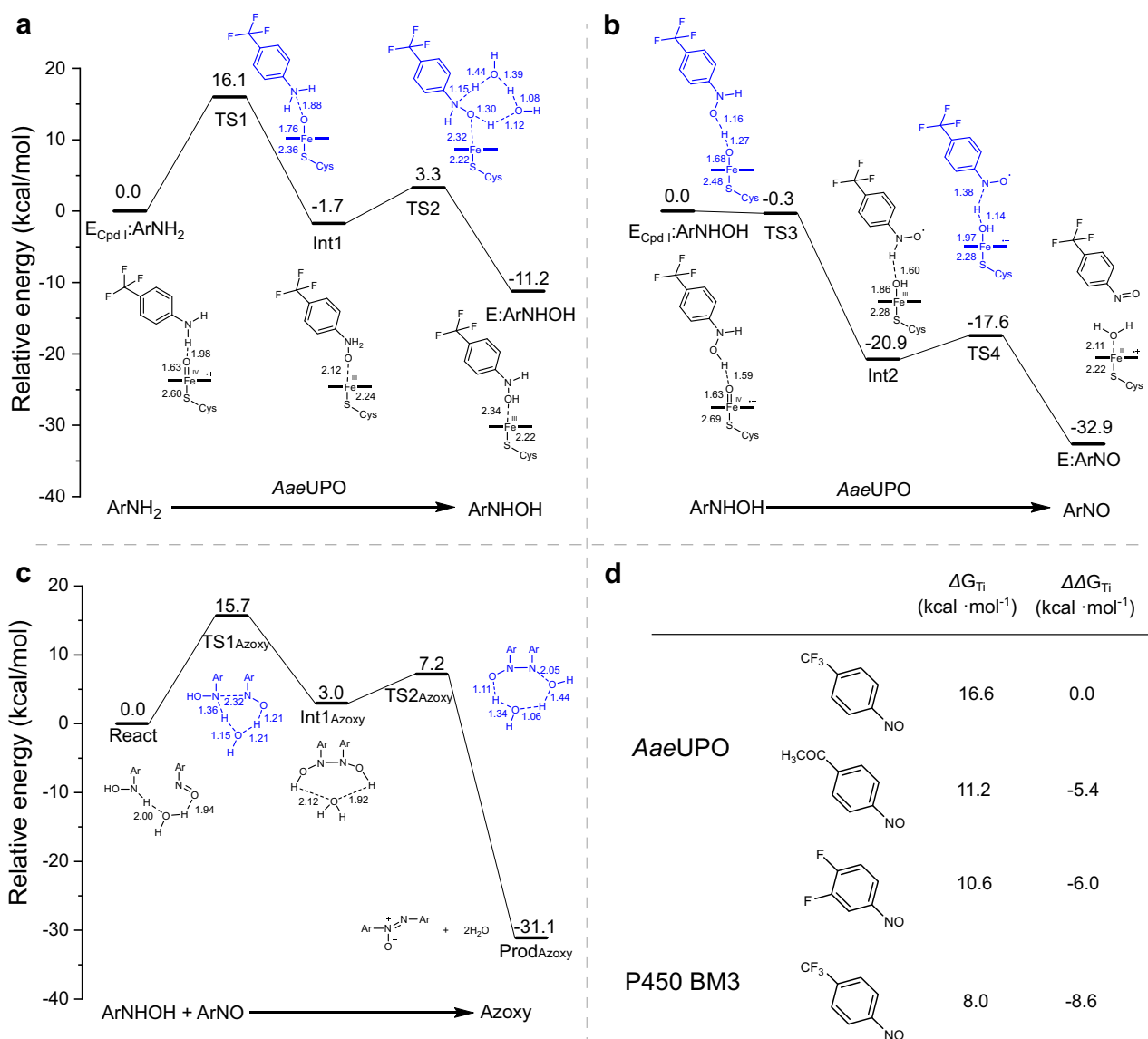
Fig. 5 | Mechanistic study of the AaeUPO-catalyzed azoxy compound synthesis from aniline. The energy profiles for the catalytic oxidation of \text{ArNH}_2 to \text{ArNHOH} (a), the subsequent oxidation of \text{ArNHOH} to \text{ArNO} (b), the formation of
