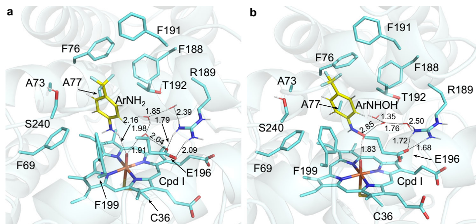
Fig. 4 | The interactions between the substrate and active site residues. Representative conformations from MD simulations for the enzyme in complex with \text{ArNH}_2 (a) and \text{ArNHOH} (b) in the presence of Cpd I. For clarity, most of the non-polar hydrogen atoms are omitted. Key distances are shown in angstroms.
