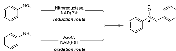
c: Envisioned enzymatic oxidative azoxy bond formation
