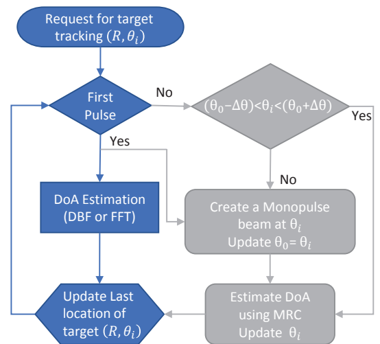
Fig. 1. Flow diagram of proposed MIMO-monopulse target tracking (grey flow) as an alternative or parallel to the tradition processing (blue flow).
