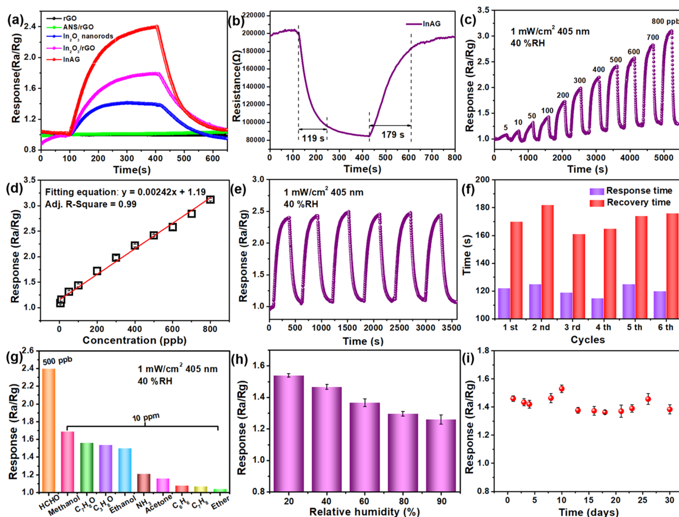
Figure 4. (a) Typical responses of rGO, ANS/rGO, In 2 O 3 nanorods, In 2 O 3 /rGO, and InAG after exposure to 500 ppb HCHO. (b) Response/recovery characteristics of InAG before and after exposure to 500 ppb HCHO at RT. (c) Real-time response curves of the InAG sensor toward different concentrations of HCHO at RT and (d) corresponding linear relationship between concentration and response. (e) Repeatability of InAG nanohybrids toward 500 ppb HCHO at RT and (f) corresponding response/recovery times for each cycle. (g) Selectivity of the InAG sensor toward 500 ppb HCHO and 10 ppm of various interfering gases. (h) Sensor response toward 100 ppb HCHO in the relative humidity range 20–90% RH. (i) Long-term stability of the sensor toward 100 ppb HCHO for up to one month at RT.
