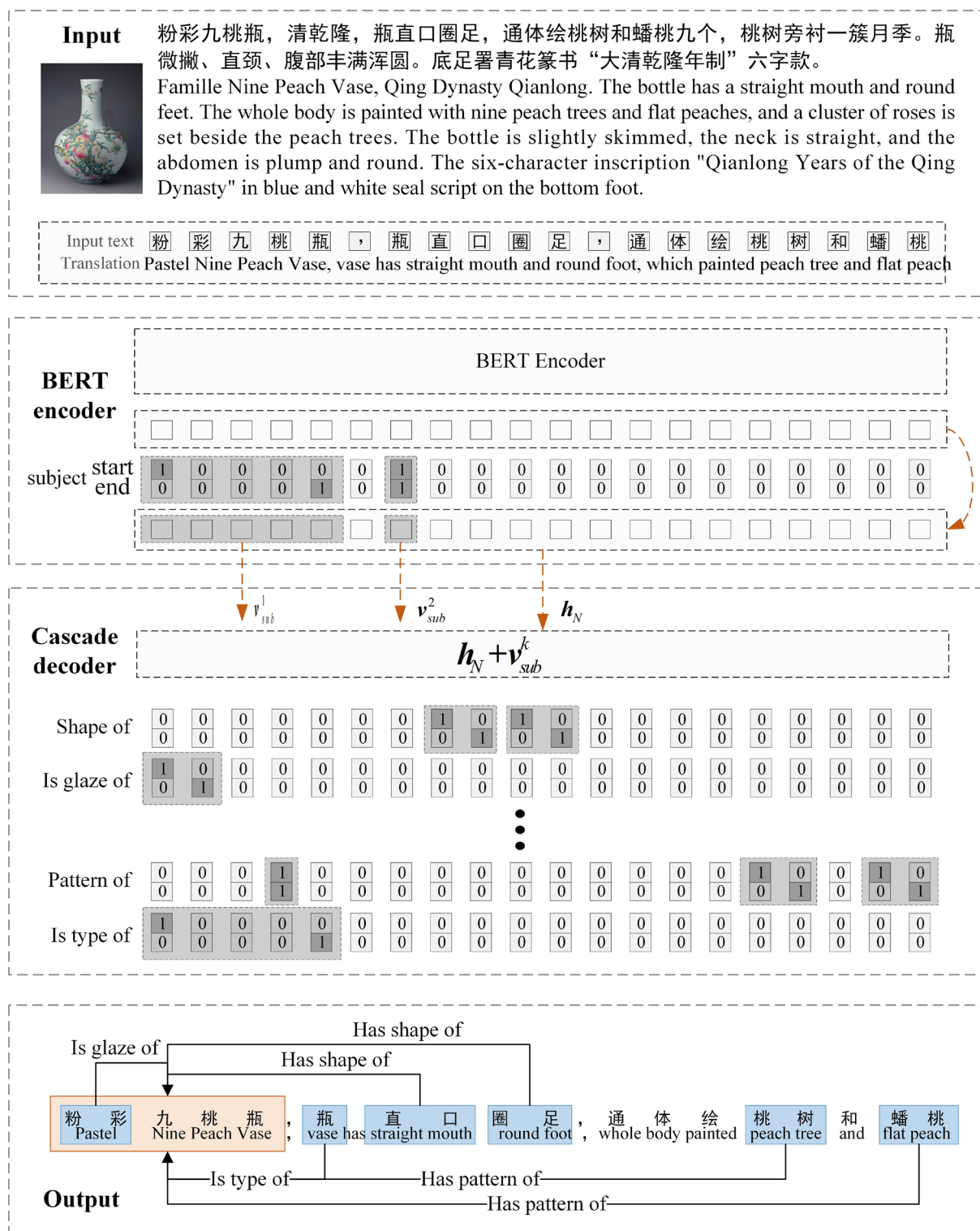
Fig. 3 Knowledge extraction model. The text in orange is the subject, and the text in blue represents an object. The lines with arrows are relationships between subjects and objects
