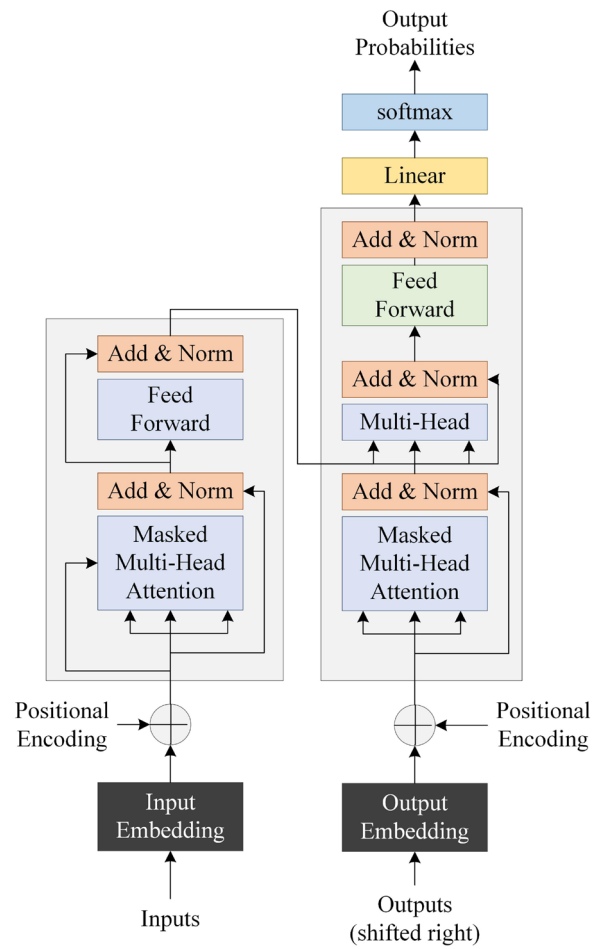
Fig. 4 The transformer framework in BERT pre-training model
