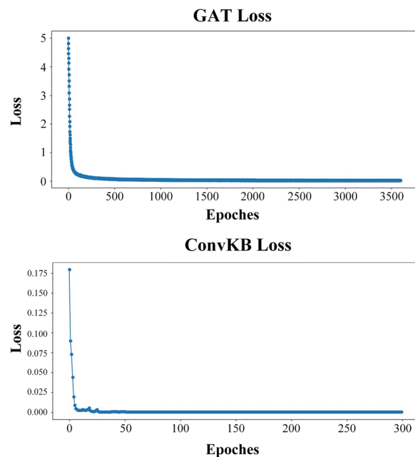
Fig. 13 Training process of knowledge completion model
