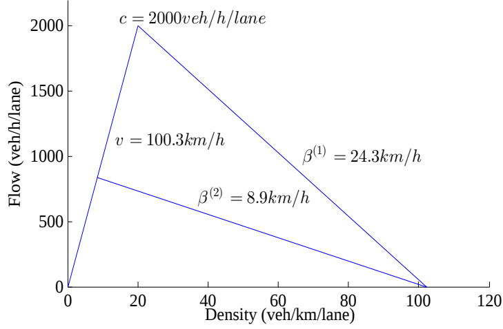
Figure 9: The calibrated fundamental diagram of controller 3
