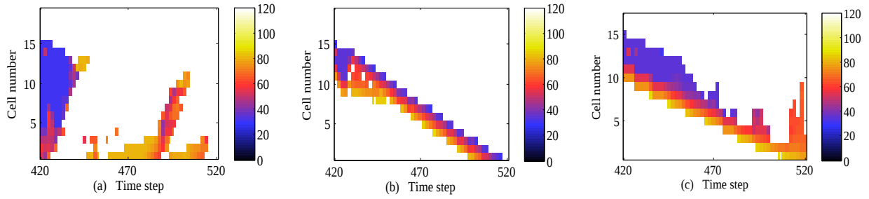
Figure 13: The VSL control signals (km/h) generated by controller 1 (a), controller 2 (b), and controller 3 (c).
