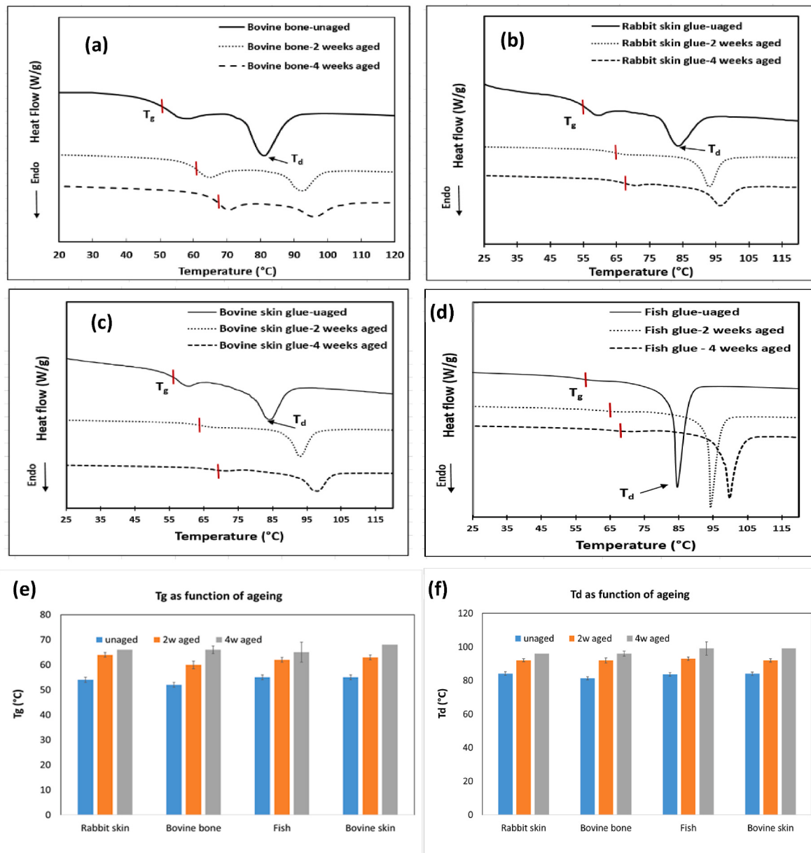
Fig. 4. (a–d) Heating DSC thermograms of unaged as well as 2 and 4 weeks hygrothermally aged animal glues after being acclimatised at 23 °C and 50% RH, prior to testing. (e–f) The increasing values of T_g and T_d of different adhesives with ageing, the error bars represent standard deviation.
