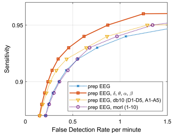
Fig. 4. Sensitivity versus FDR/min for the best features from each family (prep EEG, sub-bands, DWTs, and CWTs).
