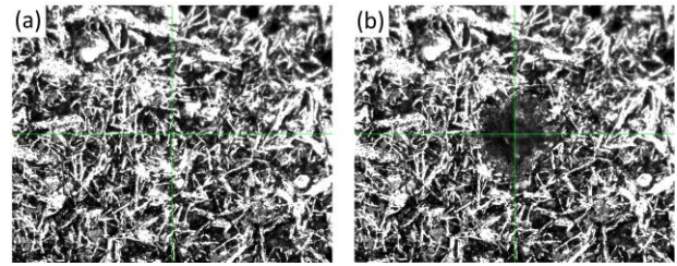
Fig. 2. Appearance of the inner structure of a Sishen particle (400 \times ) (a) before hardness test (b) after hardness test.
