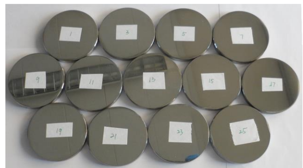
Fig. 7. Samples of mild steel disk for pin-on-disk wear test.
