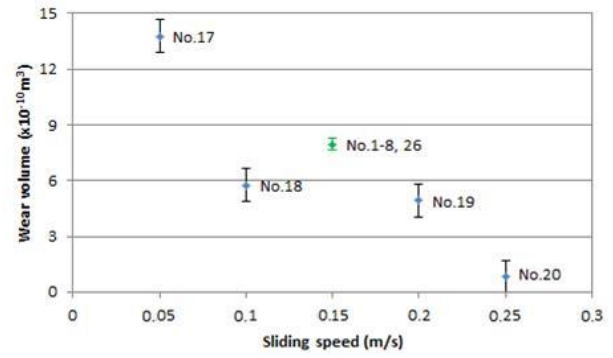
Fig. 18. Wear volume of particles as a function of sliding speed.
