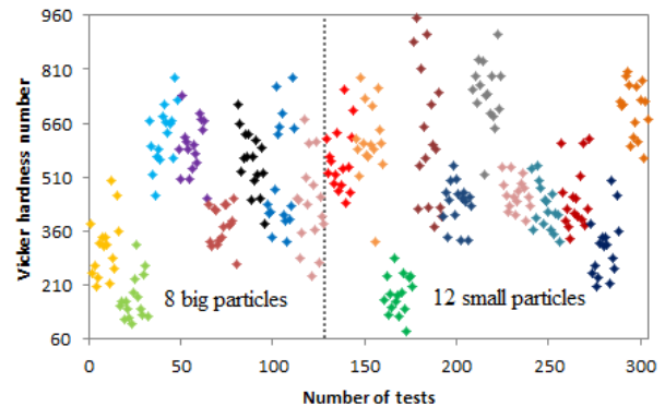
Fig. 3. Sishen particle hardness from 320 tests using 8 big and 12 small sizes.
