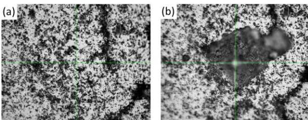
Fig. 15. Hardness test of the worn particle of No. 14 (400×) (a) appearance of inner structure before hardness test (b) after hardness test.
