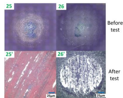
Fig. 9. Morphologies of spherical particle tips before tests (No. 25-26) and after tests (No. 25'-26').
