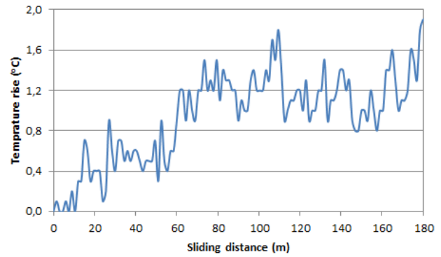
Fig. 25. Evolution of contact temperature rise for test No. 26.
