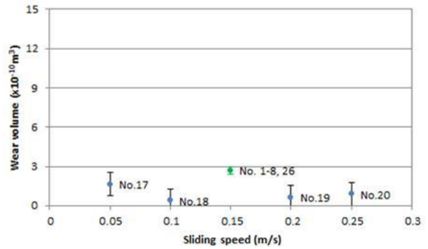
Fig. 19. Wear volume of mild steel disks as a function of sliding speed.
