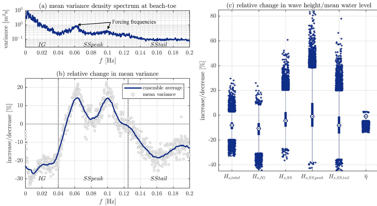
Figure 6. (a) Mean variance density spectrum at beach-toe (averaged over all simulations). (b) Relative change in mean variance at the beach-toe due to the presence of the pit \left( \frac{\sum_{i=1}^N S_{pit,i}(f)}{\sum_{i=1}^N S_{no\ pit,i}(f)} \right) (grey dots). The purple line shows the ensemble average of the points. The three frequency bands (IG, SS peak, and SS tail) are also indicated. (c) Box plots of the relative change in nearshore significant wave heights and mean water level at the beach-toe due to the presence of a pit, by comparing identical reefs with and without pit. Mean values are represented by the black dots in the white circle. The 25th and 75th percentiles are indicated by the edges of the narrow purple boxes. The purple thin whiskers extend to 1.5 times the interquartile distance, outside of which outliers are shown as purple dots.
