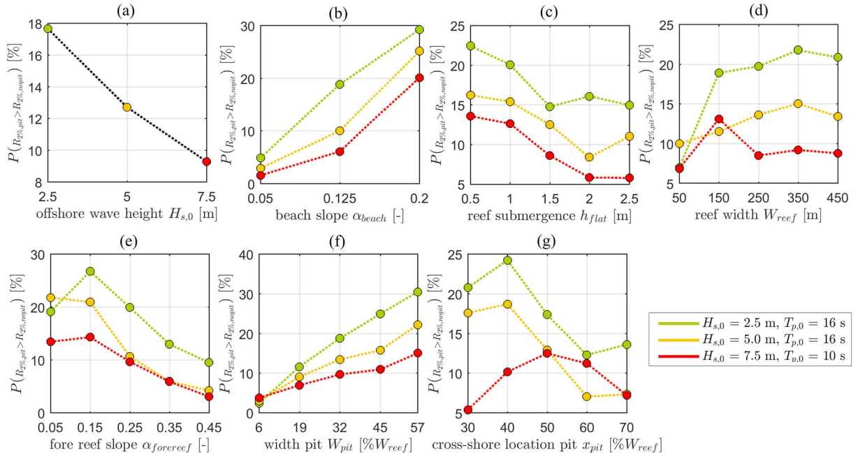
Figure 8. (a–g) Probabilities on an increase in runoff as a function of the modeling parameters. Each modeled wave condition is plotted in a different color (swell conditions with a return period of 1 (green) and swell (yellow) and tropical cyclone (red) conditions with a return period of 50 years).
