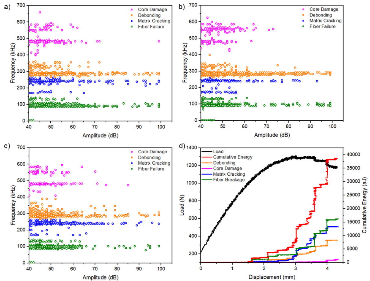
Fig. 7 Peak frequency/Amplitude data of a) N-PU, b) 0.1CNT-PU, c) 0.1CNC-PU.
