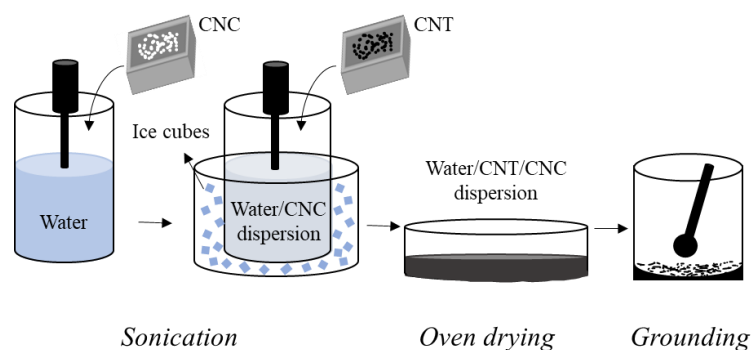
Fig. 1 CNT/CNC dispersion procedure including sonication, oven drying and grounding processes.
