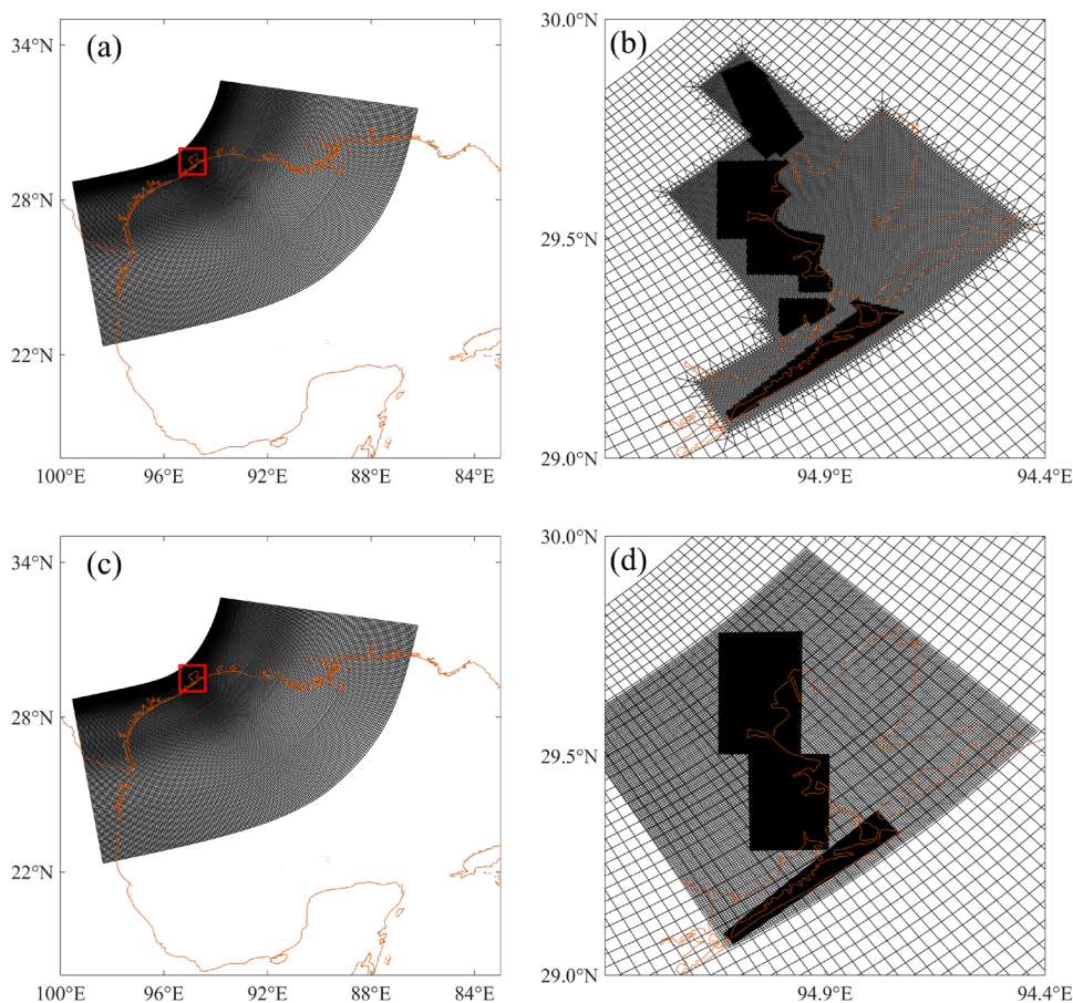
Fig. 3 Combination of triangular and curvilinear grids for the flow model and nested computational grid for the wave model. a The overall schematic of the grid, the red box is the study area where the grid is refined; b the refined area; c the coarse wave grid; d the middle and fine wave grid
