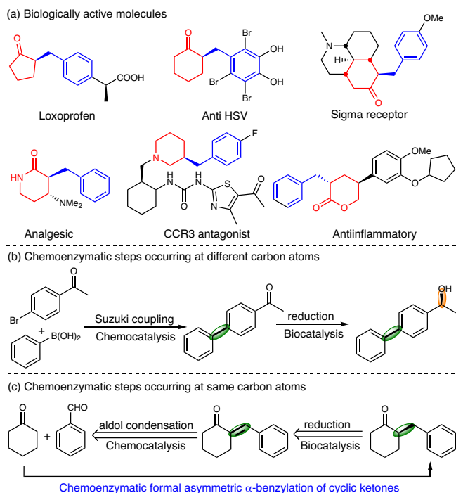
Fig. 1 | Design of a chemoenzymatic cascade for the synthesis of chiral \alpha -benzyl cyclic ketones. a Selected examples of biologically active molecules bearing \alpha -benzyl (blue) and cyclic carbonyl (red) groups. b Chemoenzymatic cascade with bond formation (green-shaded bond) and stereocenter generation (orange-shaded bond) occurring at different carbon atoms. c Chemoenzymatic cascade with bond formation and stereocenter generation occurring at same carbon atoms for formal asymmetric \alpha -benzylation of cyclic ketones.
