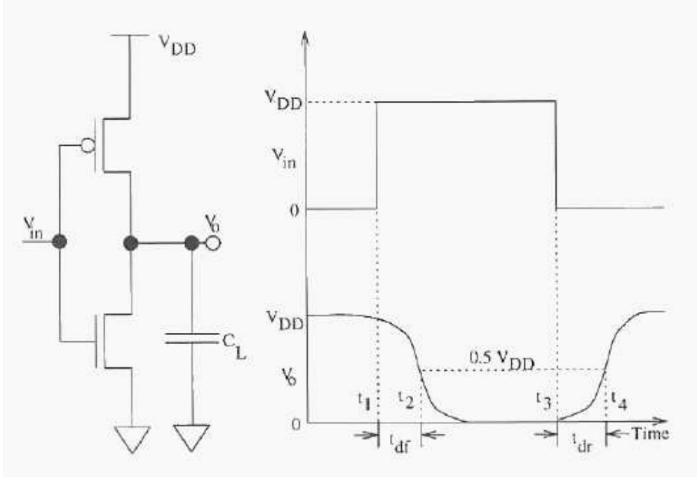
Figure 4.1: A CMOS inverter and the voltage waveforms while switching
