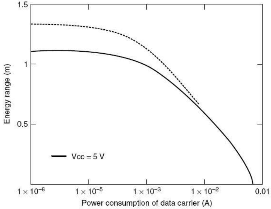
Figure 2.2: Energy range of a tag with respect to its power consumption.
