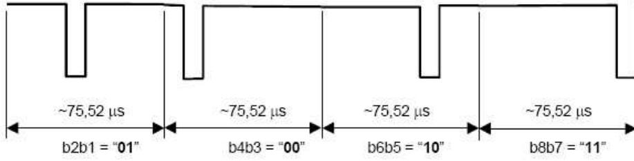
Figure 2.4: Representation of 225 in 1 out of 4 encoding
