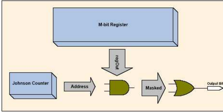
Figure 4.6: Implementation of a low-power shift register
