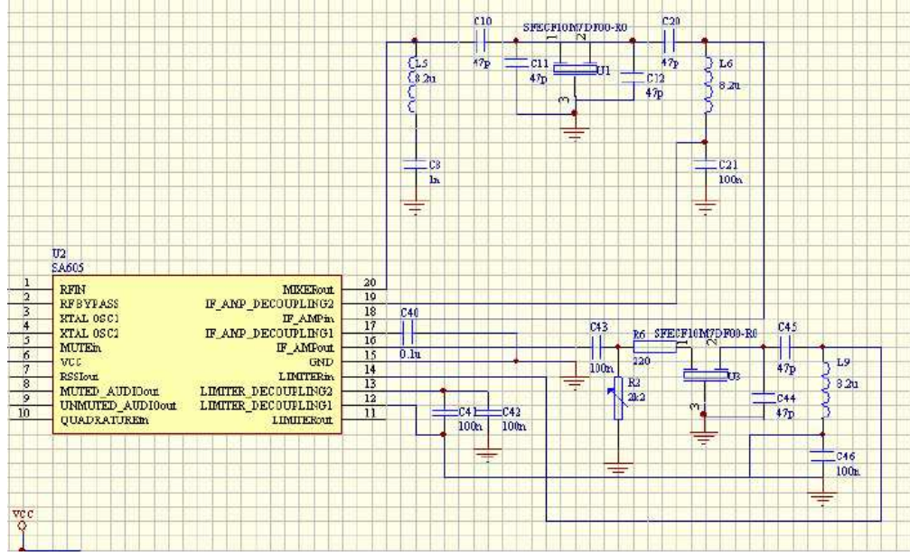
Figure 2.8: The SA605 chip and the IF filtering circuitry
