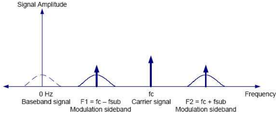
Figure 2.1: Frequency spectrum resulting from load modulation with subcarrier technique
