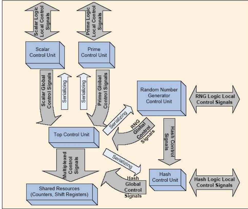
Figure 4.2: Hierarchical architecture of control unit for EllipticCore
