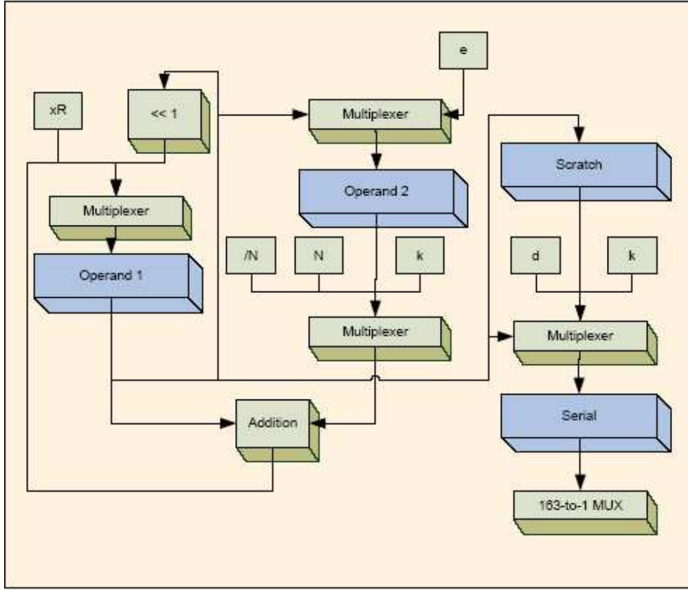
Figure 4.8: Block Diagram of the Prime Field Module
