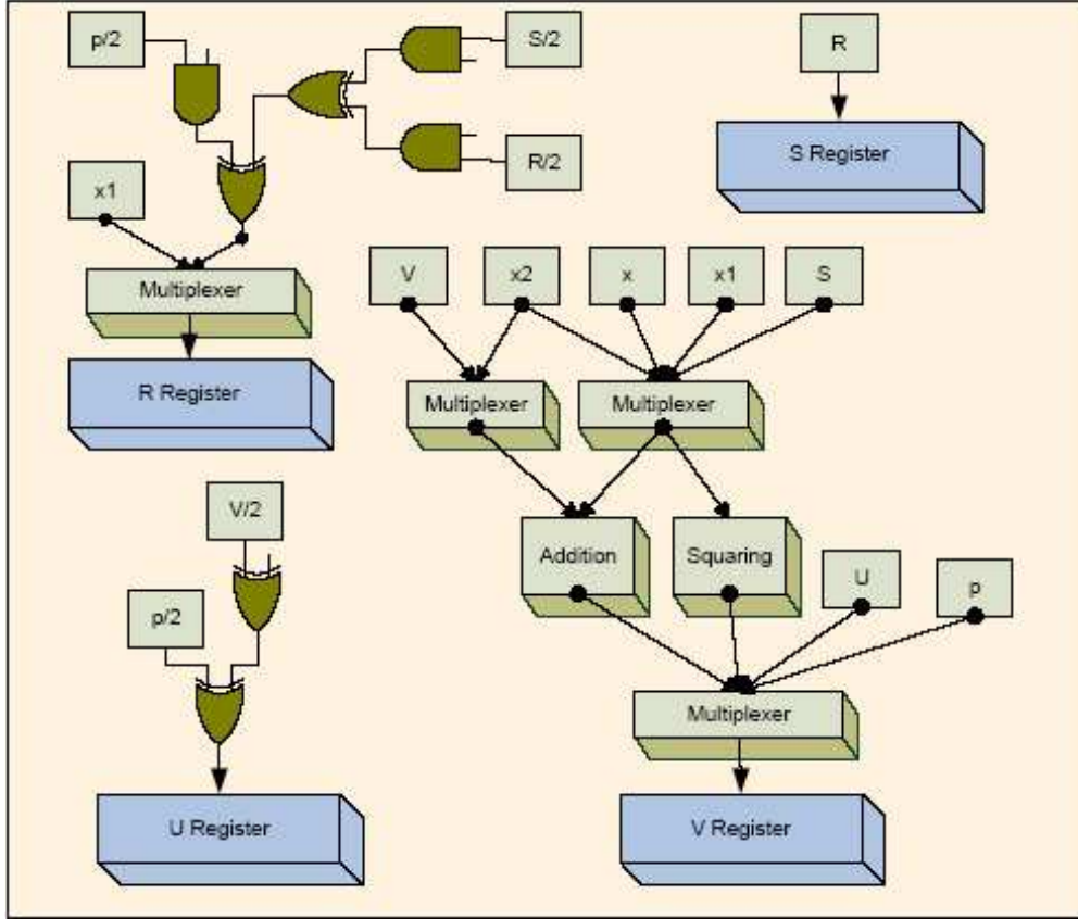
Figure 4.7: Block Diagram of the Scalar Arithmetic Unit
