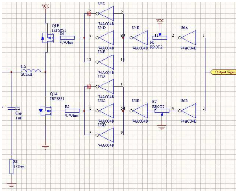
Figure 2.11: Class D power Amplifier
