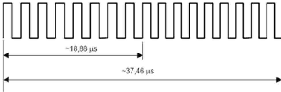
Figure 2.5: Representation of Logic 0 using a single subcarrier.
