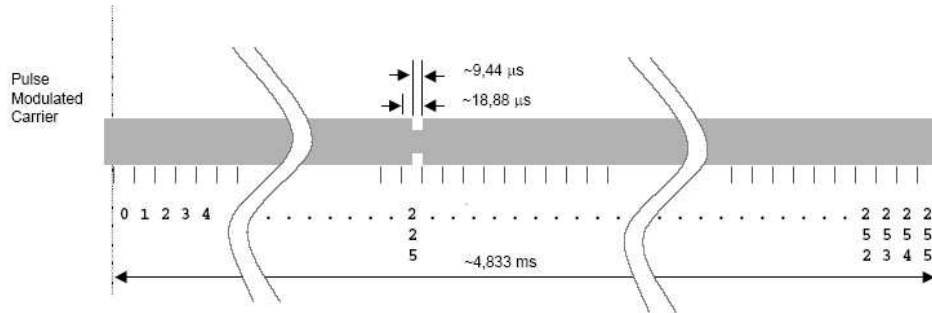
Figure 2.3: Representation of 225 in 1 out of 256 encoding
