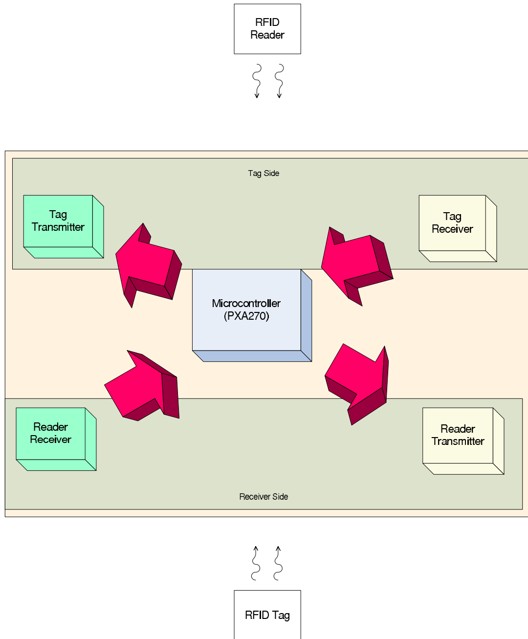
Figure 2.7: Block Diagram of the platform for the RFID Guardian
