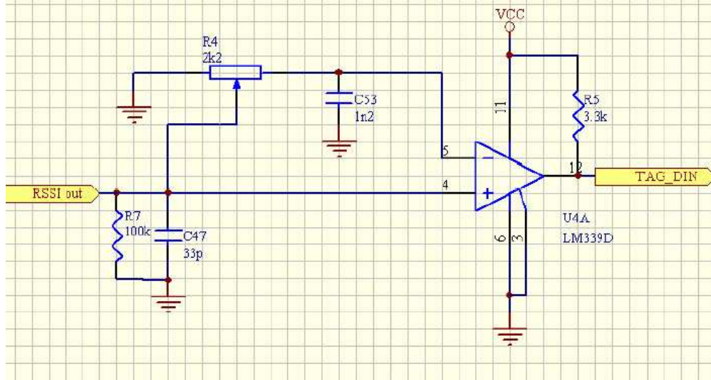
Figure 2.9: Data slicer circuit
