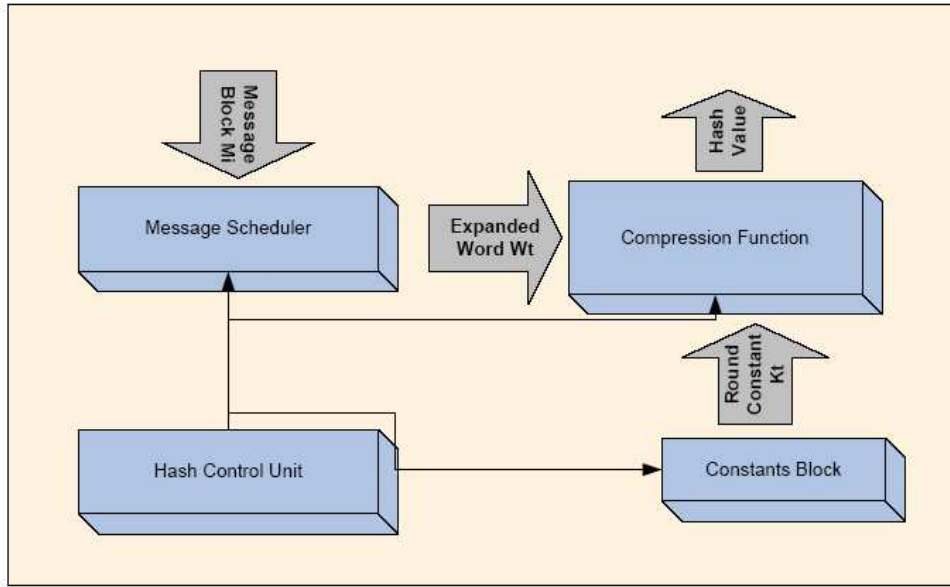
Figure 4.4: Block Diagram of the hash Unit
