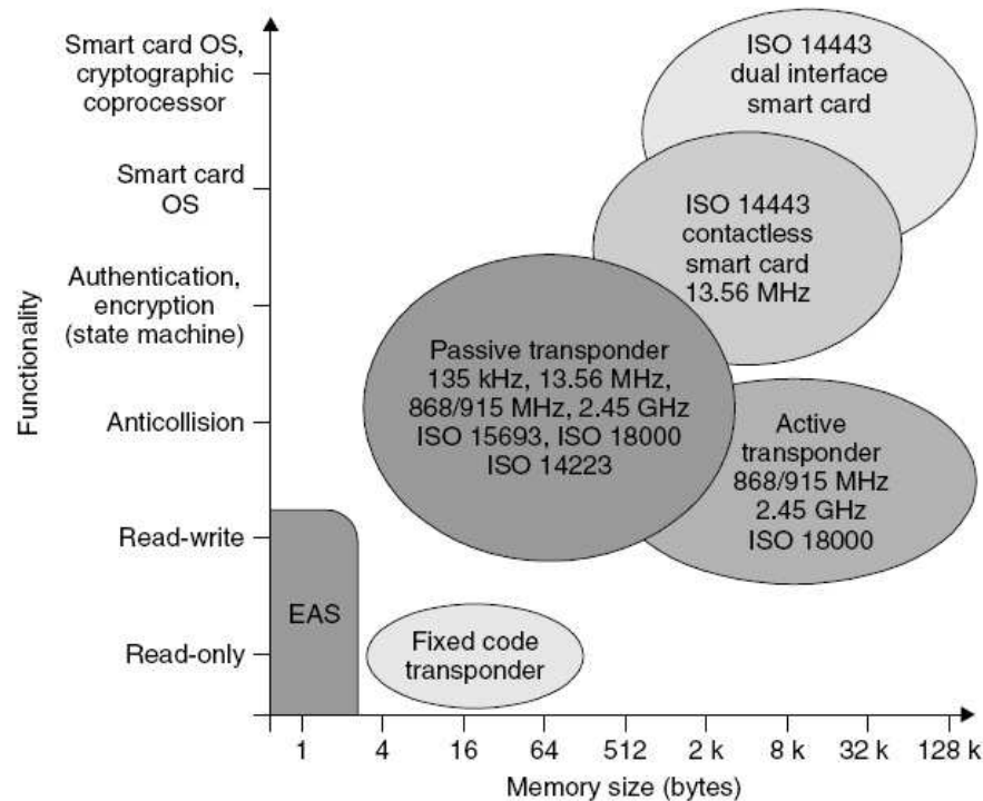
Figure 1.1: Classification of RFID systems according to their functionality
