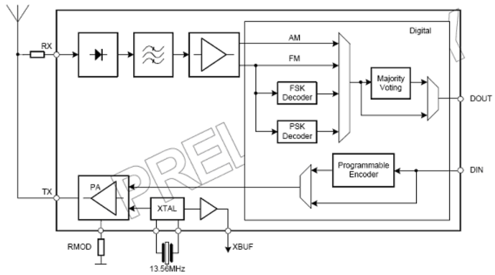
Figure 2.12: Melexis MLX90121 Block Diagram
