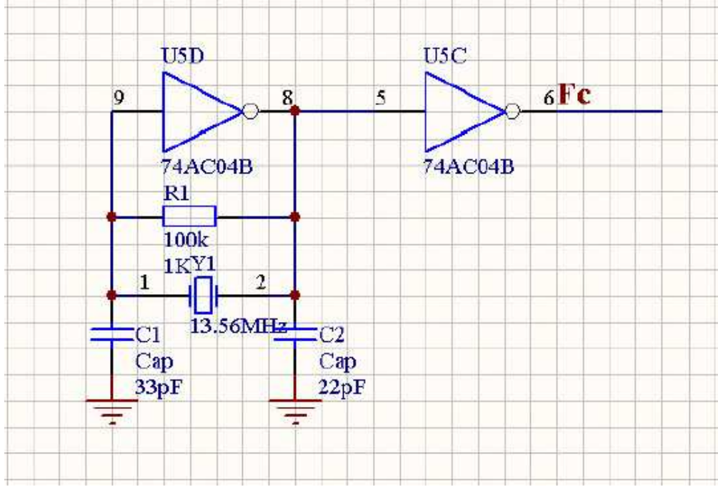
Figure 2.10: Pierce oscillator with a 13.56 MHz crystal
