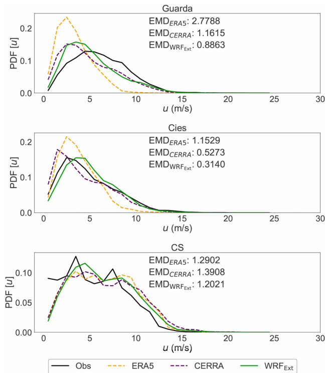
FIG. 5. Comparison of 10 m wind speed distributions from ERA5, CERRA, and WRF Ext datasets, with respect to the buoy observations, at locations: Guarda (first row), Cies (second row), and CS (third row). The EMD is calculated and shown, assessing dissimilarities between the datasets and observational data.
