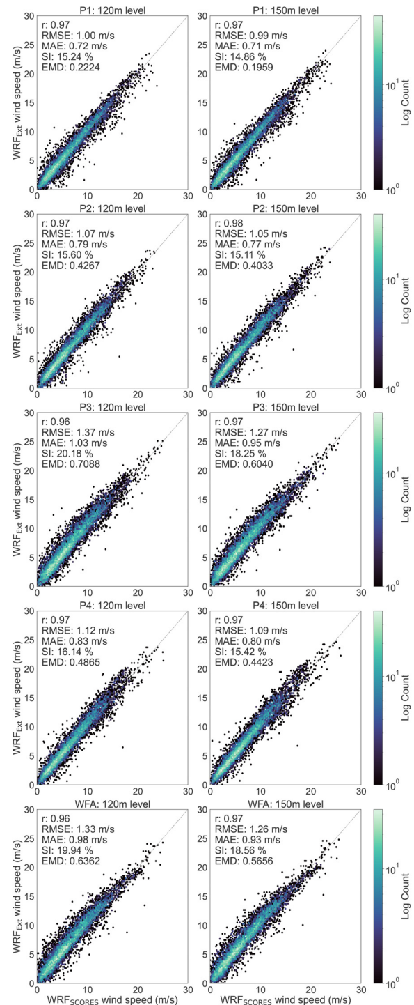
FIG. 6. Bivariate histograms depicting the 120 m (column 1) and 150 m (column 2) wind speed distributions from WRF SCORES and WRF Ext simulations, at points P1 (row 1), P2 (row 2), P3 (row 3), P4 (row 4), and WFA (row 5), during the period from 01-07-2011 to 01-07-2012, covering a year-long duration. The evaluation statistics (RMSE, r , MAE, SI, and the EMD) are computed to assess the agreement between the two datasets.
