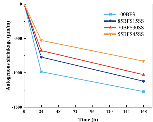
Fig. 17. Calculated autogenous shrinkage of AAS-SS pastes.
