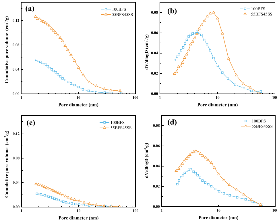
Fig. 11. Pore volume and pore size distribution curves of 100BFS and 55BFS45SS pastes: (a) and (b) for samples at 1 d while (c) and (d) for samples at 7 d.
