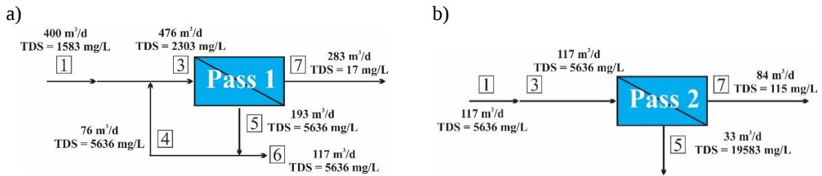
Fig. 6 (a) Primary (pass 1) and (b) secondary (pass 2) RO tandem system configuration. Numbers and associated conditions are for the dry season; they are explained in Table 4. Stream 1 in pass 2 comes from stream 6 in pass 1. Streams 2, 4 and 6 are not displayed in case of no recirculation.
