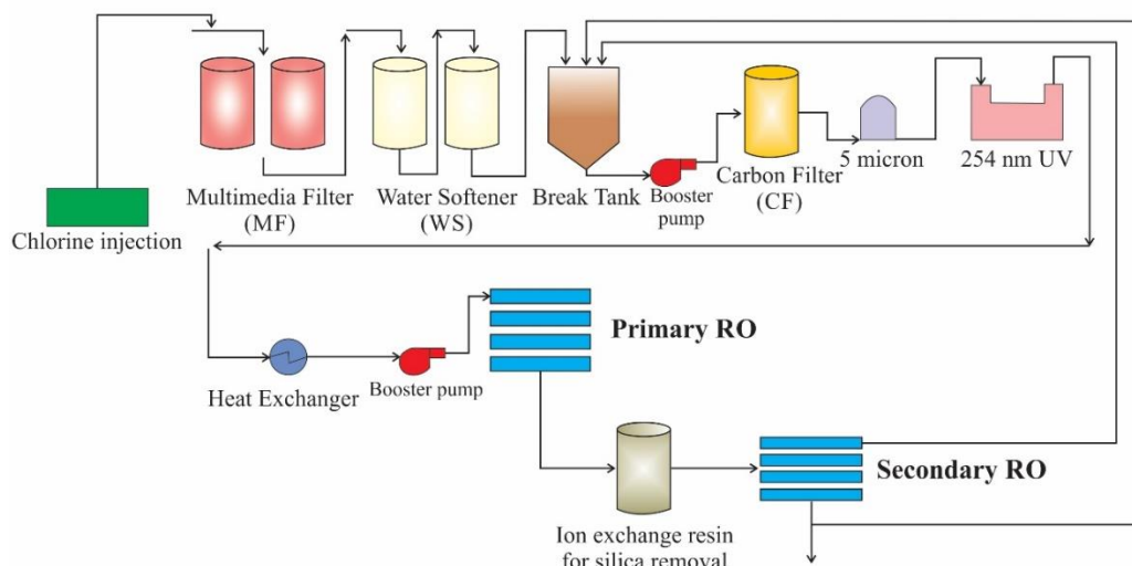
Fig. 1. Process flow diagram of the proposed treatment system design. The intermediate treatment stage (silica removal ion exchange resin) is optional depending on SiO 2 concentration.
