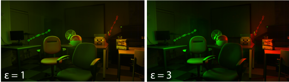
Figure 2.5: Shepard interpolation of captured sources varying \varepsilon .
